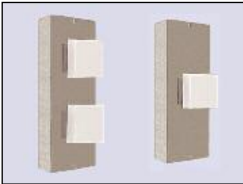
WLP-2 VCS - Intermediate WLP-1 VCS - Terminal Box: 4.50"W x 13"H x 2.50 Deep Lens centerline: 6.0". Coverless Lantern with 4" Sq. Lenses and Plaster ring (1.250" long) for dry wall applications. Custom lenses available - call for information. Wall cutout: 3.562" Sq.
