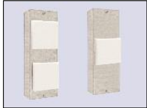
WL-2 VCS - Intermediate WL-1 VCS - Terminal Box: 4.50"W x 13"H x 2.500" Deep Lens centerline: 6.0". Coverless Lantern with 4" Sq. Lenses Custom lenses available - call for information. Wall cutout: 3.500" Sq.
