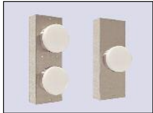
WLP-2 VCR - Intermediate WLP-1 VCR - Terminal Box: 4.50"W x 13"H x 2.50 Deep Lens centerline: 6.0". Coverless Lantern with 4" Dia. Lenses and Plaster ring (1.250" long) for dry wall applications. Custom lenses available - call for information. Wall cutout: 3.562" Dia.
