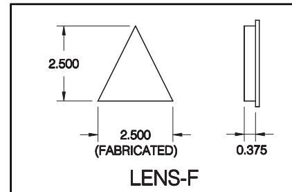
Part #: A474CL
