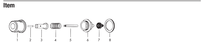
Push Button For Exposed Royal® & Crown® (Seat Action)
