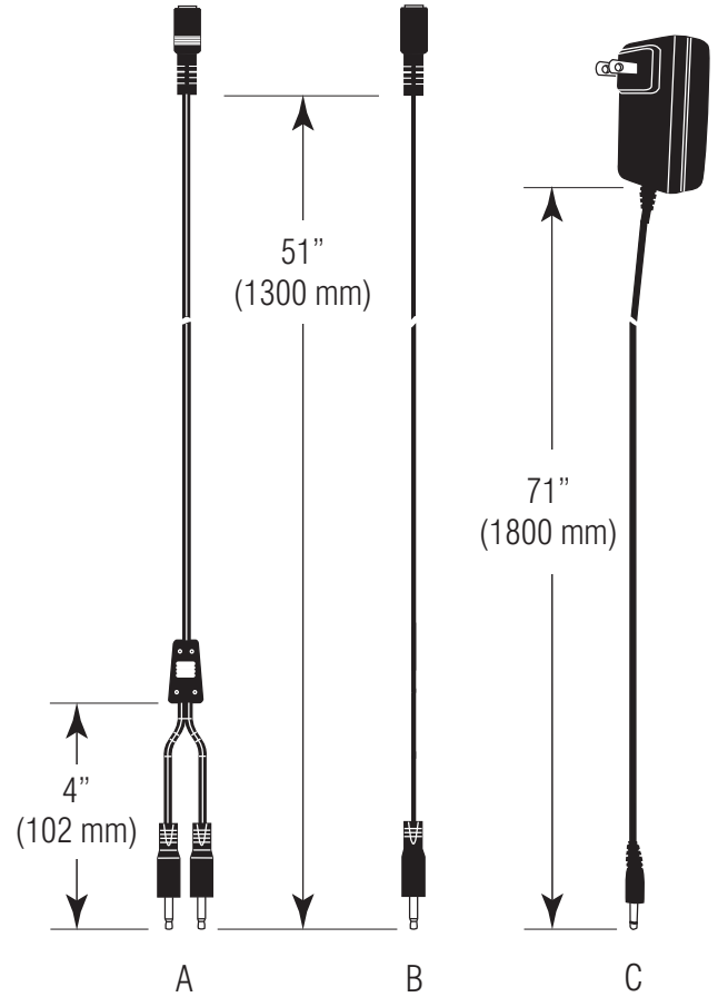
EW-62000 Double Station Cables
