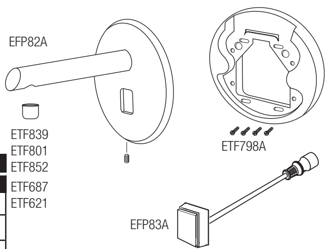
EBF-850 Wall Mount, battery ETF-800 Wall Mount, hardwired
