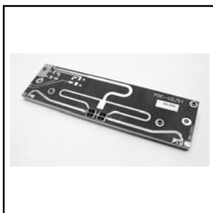
DC02N01UTA 2 WAY COUPLER 470-860 MHz, 15W Price: $135.00
