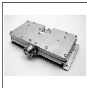
DC02N10FMA 2 WAY COUPLER 87.5-108 MHz, 1000W Price: $210.00
