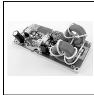
IS300-1050 10-50 MHz, 300W 52V, Gain 19dB Class A Price: $300.00
