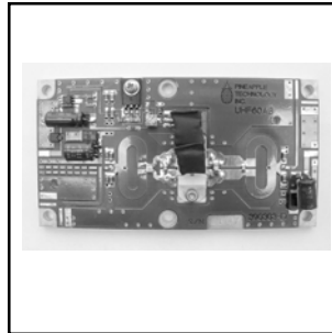
UHF60-AB UHF-TV 60W, CLASS AB, 470-860 MHz Price: $706.00
