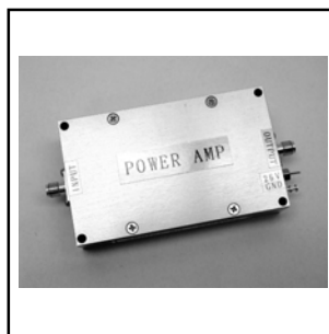
RFGL-900A 800-960 MHz P1dB 33dBm 29dB Gain Price: $230.00
