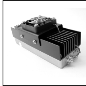
RFGA0012-05 1-2GHz, 5W Pout 38dB Gain, Class A Price: $1,400.00
