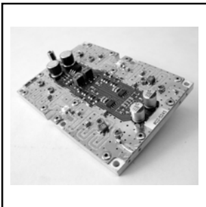
LDV05PG 134-176 MHz, LDMOS Tech., 5W CW, 7.5W@- 40dBC (two-tone) for PAGER applications Price: $290.00
