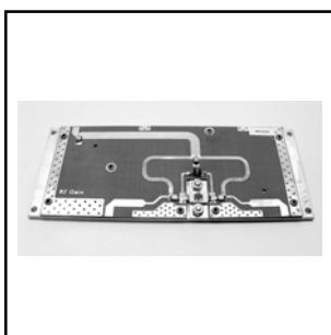
DC02N03UTA 2 WAY COUPLER 470-860 MHz, 300W Price: $199.00
