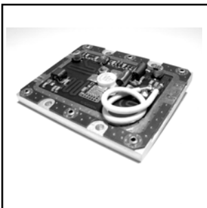
MDL30 87.5-108 MHz, 30W 28V, 17dB Gain Class AB Price: $135.00
