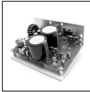
PWSS28-10 Step down, 31VAC > 25-28VDC , 8A Four-terminal, 100 kHz switching regulator with a wide-input voltage range. Price: $105.00
