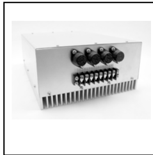
PWSS50-35 STEP DOWN , 75 VAC > 40-52 VDC , 35A , \eta > 90\% Price: $580.00
