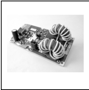
HF300-0130MC 1-30 MHz, 300 W 21 dB Gain, Class AB 50 V commercially pure copper CPA 122 plate Price: $498.00
