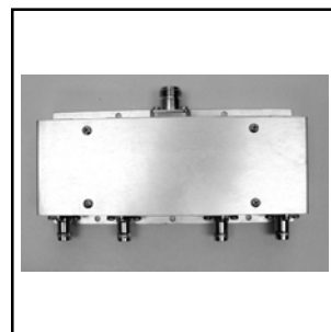
DC04Y01VLA 4 WAY COUPLER 45-120 MHz, 100 W Price: $155.00
