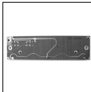
PDCU2-02 2-WAY 470-860 MHz, 100 W Price: $86.00
