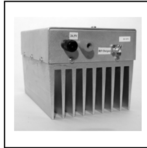
THU2600-HS 25w, 26.5v, Class A Price: $755.00
