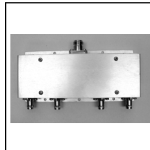
DC04Y01VHA 4 WAY COUPLER 175-225 MHz, 100W Price: $155.00
