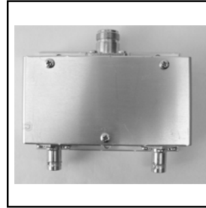
DC02Y10VLA 2 WAY COUPLER 45-120 MHz, 1000 W Price: $275.00
