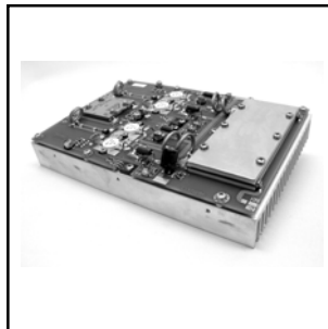
THV60 174-235 MHz, 60W, 14dB Gain, Class A, 28V Price: $850.00
