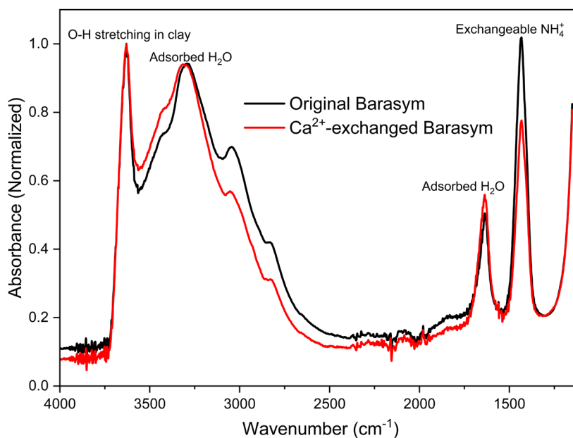
650 Figure A. FTIR spectra for original and \text{Ca}^{2+} -exchanged Barasym samples for semi-quantitative analysis of \text{Ca}^{2+} exchange with \text{NH}_4^+ .
