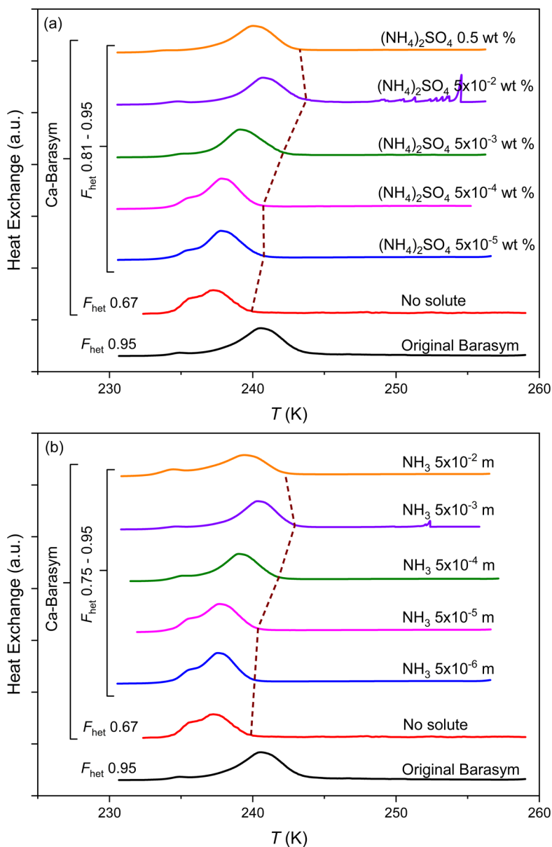
355 Figure 2. DSC thermograms obtained via emulsion freezing experiments with Barasym in pure water (original Barasym), compared with the ion exchanged Ca-Barasym in pure water and in (a) ammonium sulfate solutions (in wt %) and (b) ammonia solutions (in molality) with increasing concentration as indicated on the DSC curves. The concentration of Barasym in the suspensions was 0.5 wt %. The dashed brown line indicates the freezing onsets. All curves are normalized such that the areas under the heterogeneous and homogeneous freezing curves sum up to the same value.
