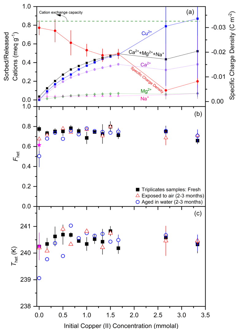
430 Figure 4. Ion exchange experiments as a function of Cu 2+ concentration in a 0.5 wt % STx-1b suspension showing the effect of the stepwise exchange of the charge-balancing cations (Ca 2+ and minor amount of Mg 2+ and Na + ) with Cu 2+ on the IN activity of the montmorillonite. Panel (a) shows sorbed Cu 2+ together with released Ca 2+ , Mg 2+ and Na + as separate curves and summed up to Ca 2+ + Mg 2+ + Na + in terms of meq/g (left scale) together with the specific charge density on the montmorillonite particle surface (right scale). The horizontal green dashed line marks the cation exchange capacity (CEC) as reported by CMS. DSC thermograms of the freshly ion-exchanged and lyophilized samples as 1 wt % suspensions in pure water have been measured in triplicates (black filled squares with error bars representing ± SD) few days after 435 preparation and been evaluated in terms of F_{het} in panel (b) and T_{het} in panel (c). A few samples have been re-measured after 2–3 months either after storage in air (red open triangles) or aged in water (blue open circles). The black square at 0 mmol Y 3+ marks the sample that was treated the same way as the ion-exchanged samples (including lyophilisation). As a reference, filled magenta stars indicate F_{het} and T_{het} of the original STx-1b in water.
