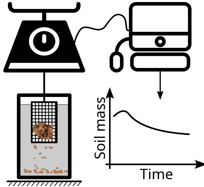
Figure 1. The QuantiSlakeTest (QST) aims at weighing an undisturbed soil sample suspended in demineralised water by means of an 8 mm mesh metallic basket. The QST device, illustrated here, consists in a balance connected to a computer for direct data-logging. The open-source application for parametrising and driving the experience and for visualising data is released as a development R-package (< https://frdvnw.gitlab.io/slaker/dev/ >). Video comparing the QST of two contrasting soil samples can be watched here: < https://youtu.be/G9UweThvHYI > – Credits : figure based on two illustrations created by Mohamed Mb from Noun Project (CC BY 3.0)
