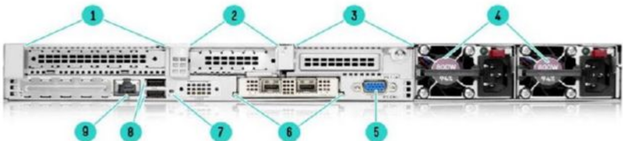
Rear View - Standard for all DL365 Gen10 Plus
