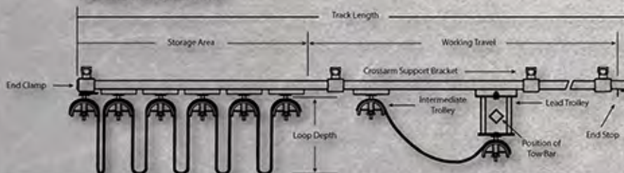
TYPICAL SYSTEM LAYOUT
