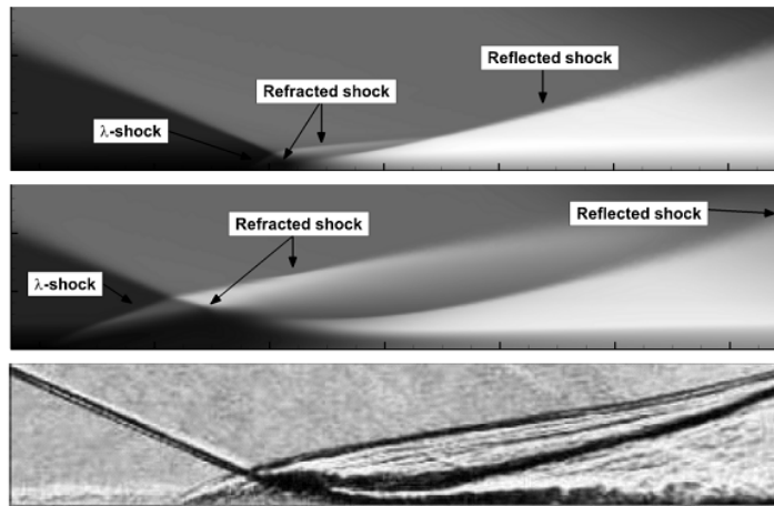
Figure 15. Density contours in comparison with the Schlieren visualization for \beta = 14^\circ (from top to bottom: SU2 SA model, SU2 k-\omega SST model and the experiment of Schülein et al. [27])
