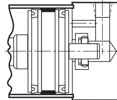
Piston and rod assembly for 1-1/2" thru 5" bore cylinders with stroke lengths of 1/2" and less than 2".
