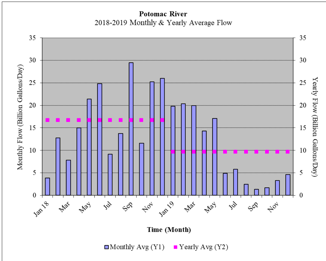
Figure 2.3 Monthly and yearly average flow on the Potomac River, 2018–2019.
