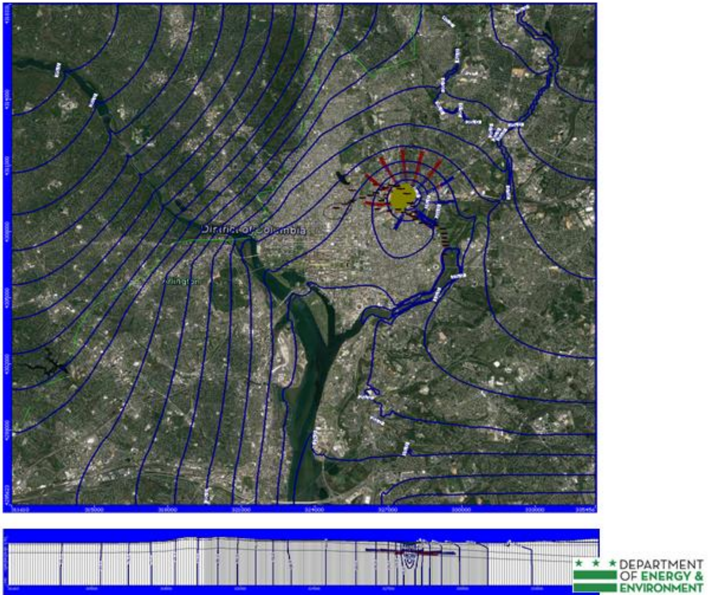
Figure 5.3 Groundwater Model and its Use for Dewatering Permits and Evaluation.
