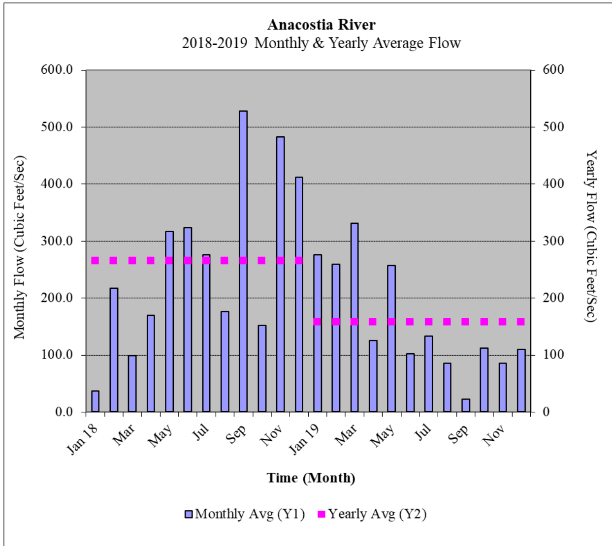
Figure 2.2 Monthly and yearly average flow on the Anacostia River, 2018–2019.
