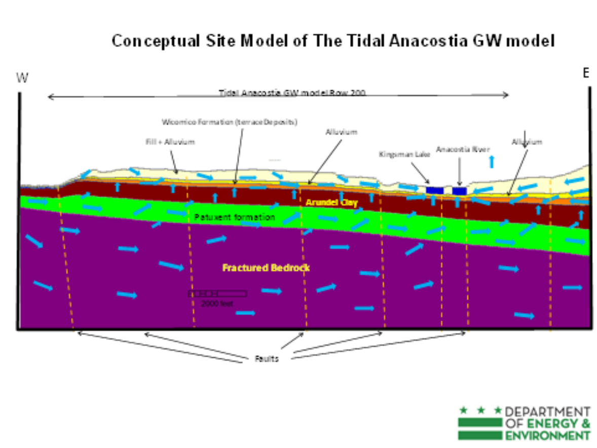
Figure 5.4 Tidal Anacostia River Groundwater Model Conceptual Site Model.
