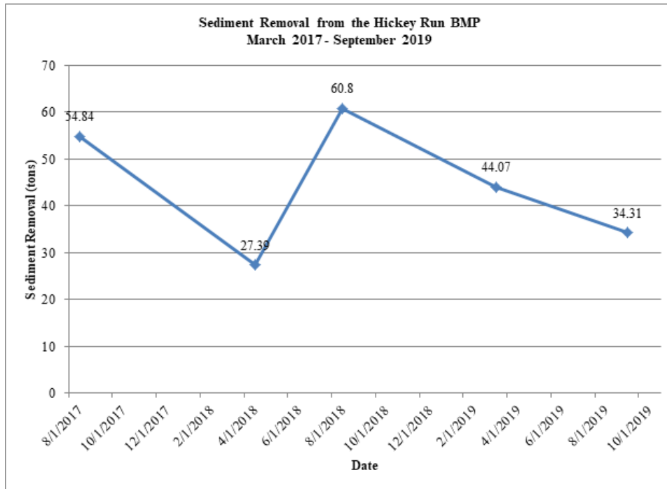
Figure 3.4 Sediment Removal from the Hickey Run BMP from March 2017 through September 2019.
