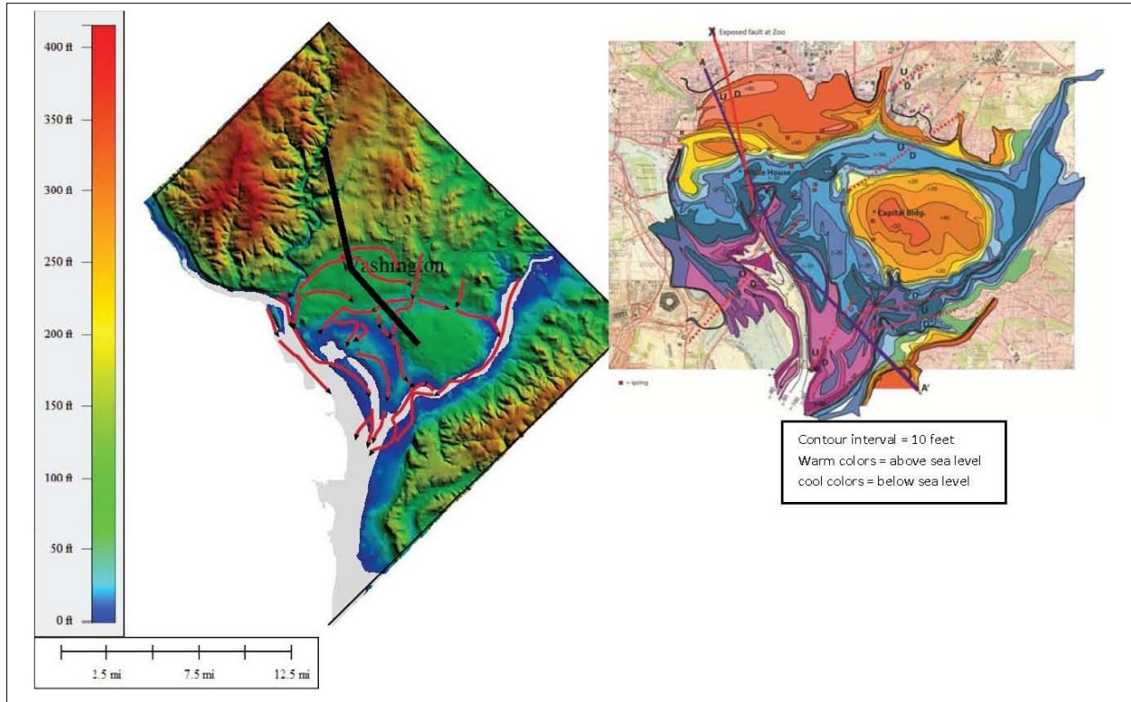
Figure 5.1 (Left) LiDAR elevation map of Washington D.C. and the paleochannels found in the current joint USGS-DOEE study (arrows pointing downriver). (Right) Structure contour map of base of Quaternary sediments showing numerous paleochannels and locations of proposed faults (red dashed lines) and documented fault (solid red line).
