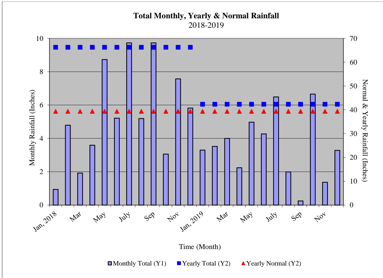
Figure 2.1 Total monthly, yearly, and normal total rainfall (inches), 2018–2019 (Source: National Weather Service, Ronald Reagan Washington National Airport).
