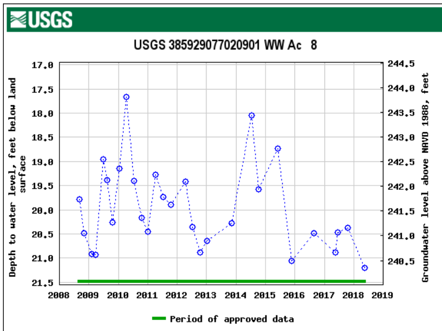
Graph of manual water-level measurements for well DCMW04-08 (WW Ac 8).
