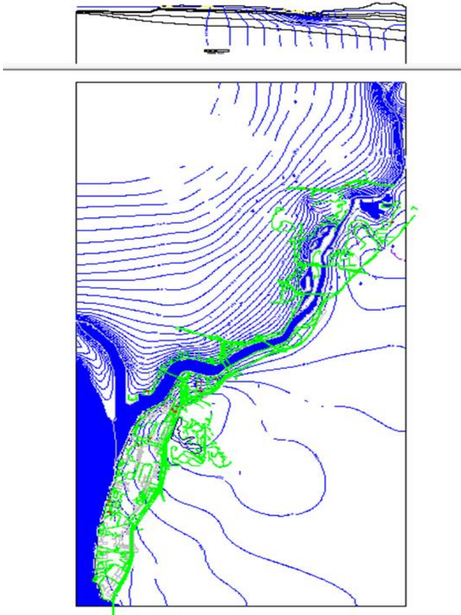
Figure 5.5 Tidal Anacostia River Model Results.
