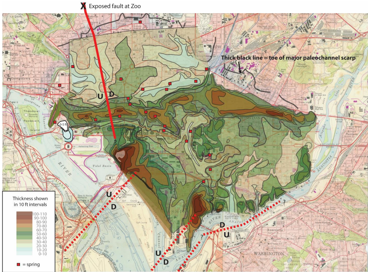
Figure 5.2 Map of the thickness of the Quaternary deposits beneath downtown Washington D.C. Thicker areas are sandy infillings of paleochannels and are groundwater reservoirs and conduits. The locations of most springs coincide with steep gradients where younger channel erosion cuts into older paleochannel deposits.
