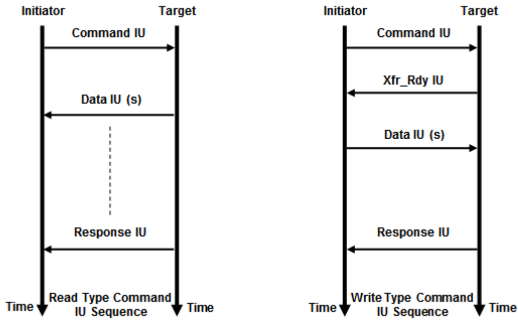
Figure 13 SSP Information Unit Sequences
