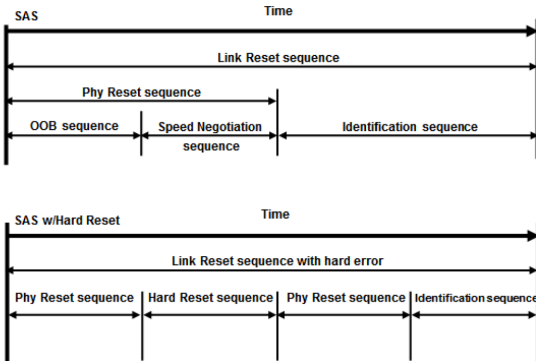
Figure 12 Link Reset Sequence
