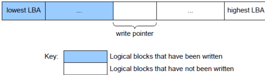
Figure 16 Write pointer zone and write pointer
