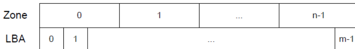
Figure 14 Zones in a zoned block device
