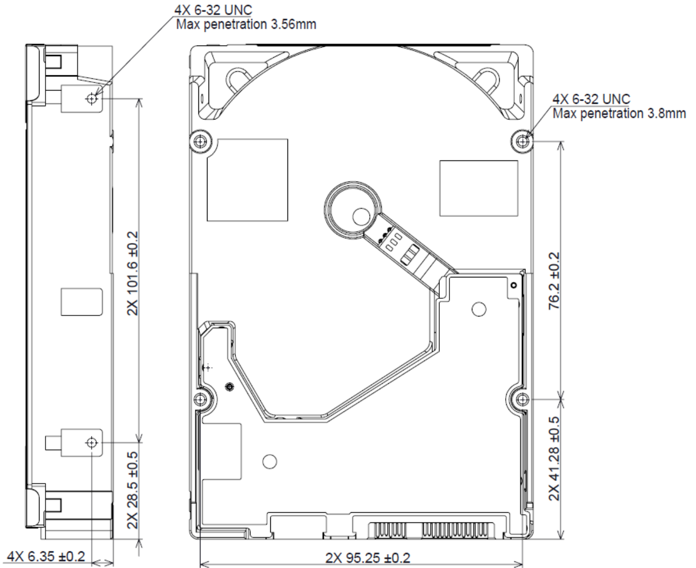
Figure 9 Bottom and side views with mounting hole locations (FIPS model)
