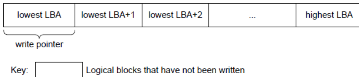
Figure 15 Write pointer zone and write pointer after reset write pointer operation with no subsequent writes
