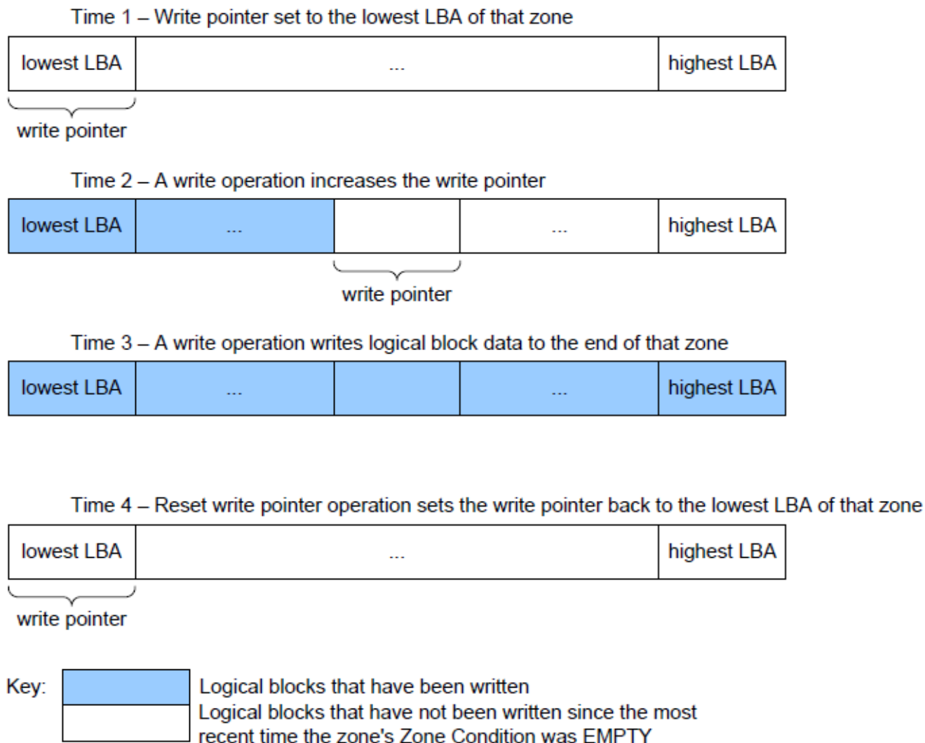
Figure 17 Write pointer zone example operations
