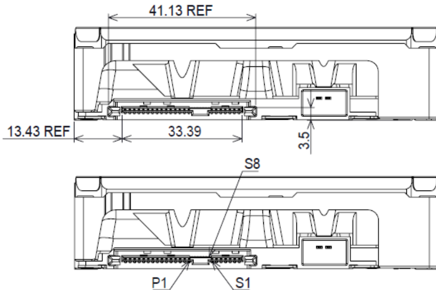
Figure 10 Connector locations
