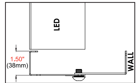
DETAIL
