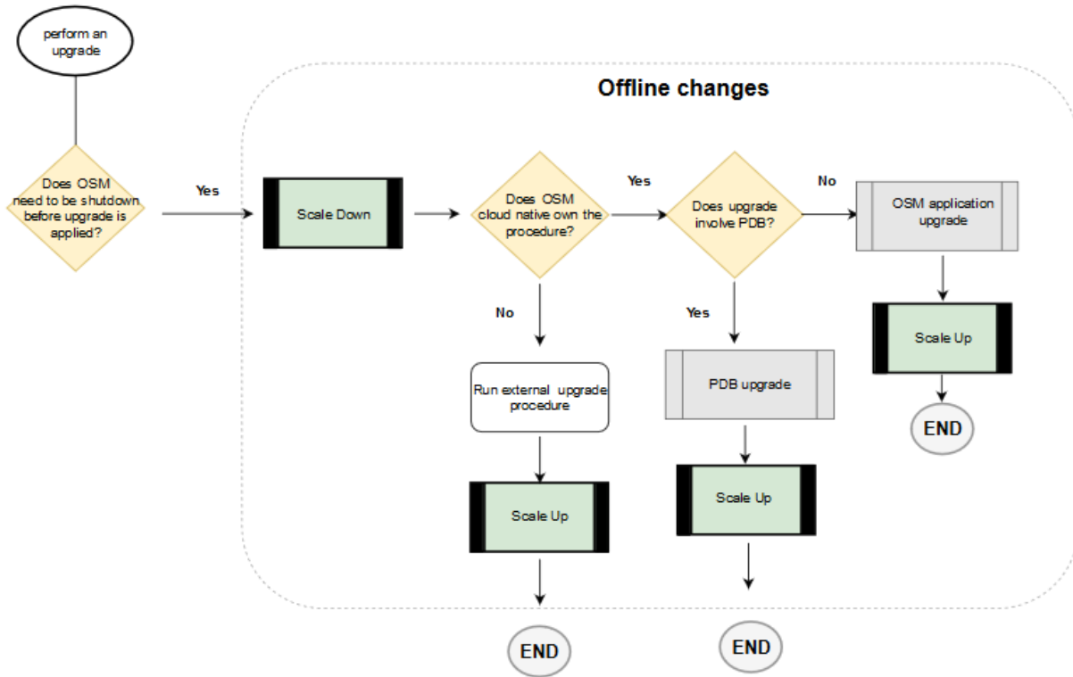
Figure 11-3 Upgrade Path Flow for Offline Changes
