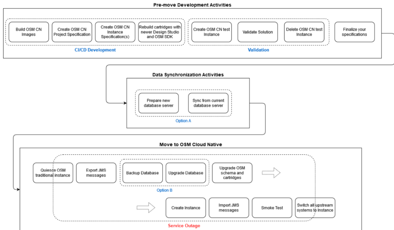
Figure 13-1 Move to OSM Cloud Native Process
