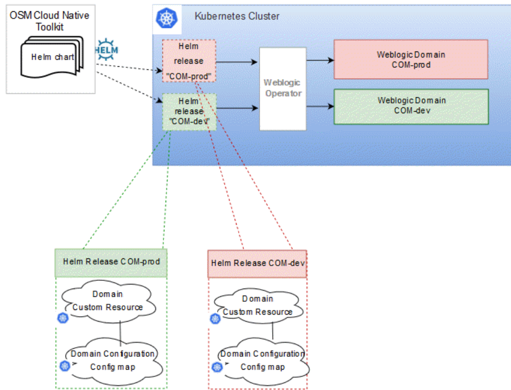
Figure 1-4 OSM Cloud Native Deployment Environment
