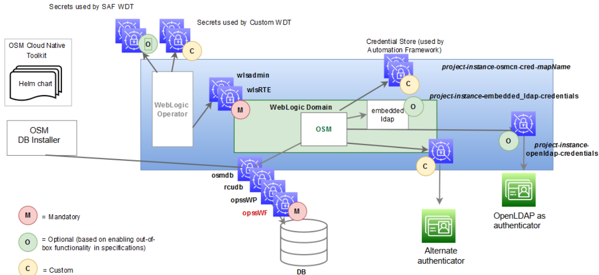
Figure 6-1 Kubernetes Secrets in OSM Cloud Environment
