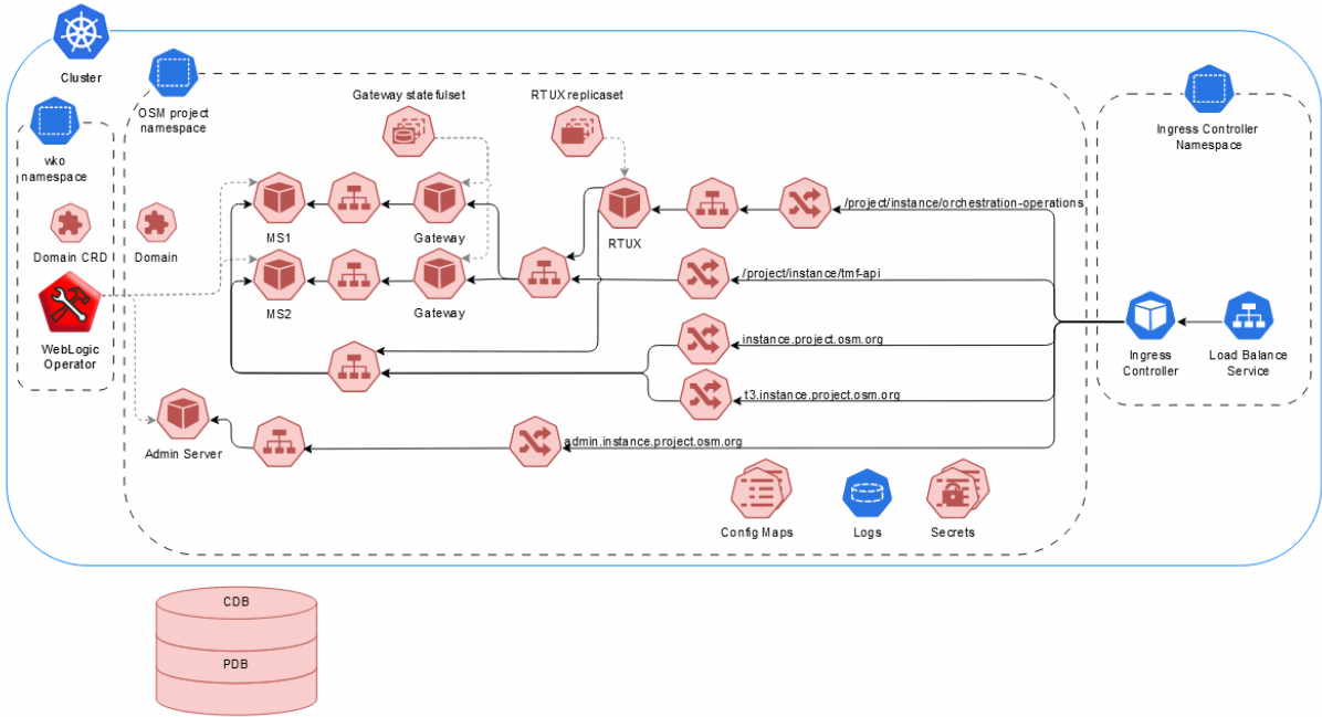
Figure 1-2 OSM Cloud native Runtime Deployment in Kubernetes
