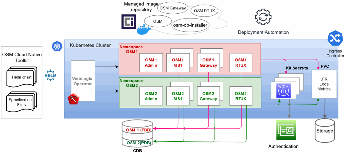
Figure 1-1 OSM Cloud Native Architecture
