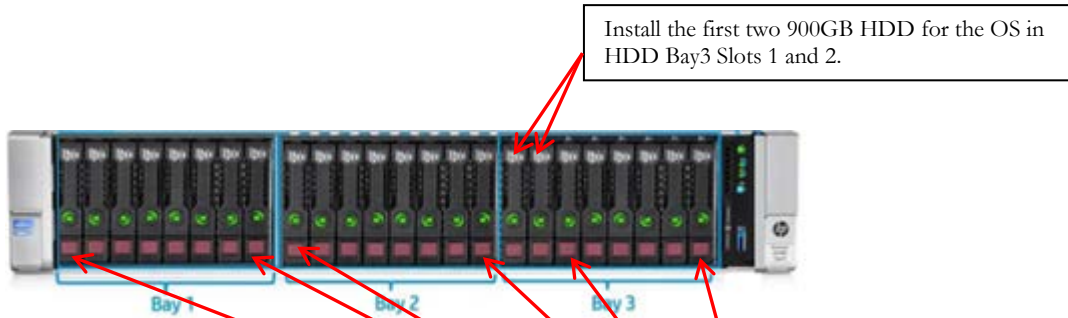
Figure 4 : Front view for HP DL38 Gen9
