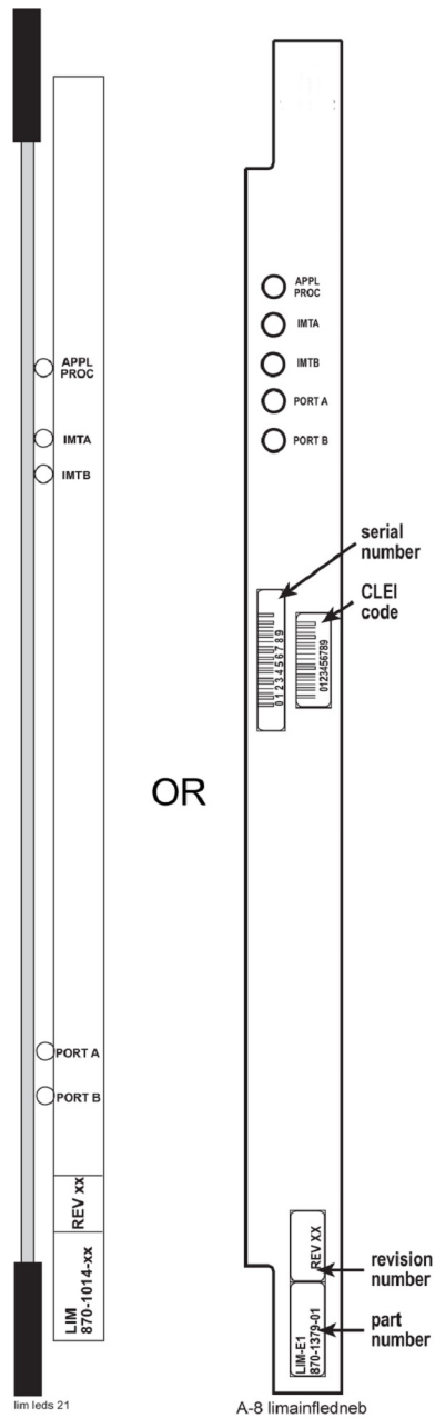
Figure 3-4 Card LEDs
