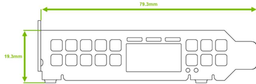
Single-port Adapter Short Bracket
