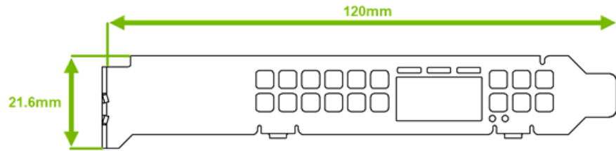
Single-port Adapter Tall Bracket
