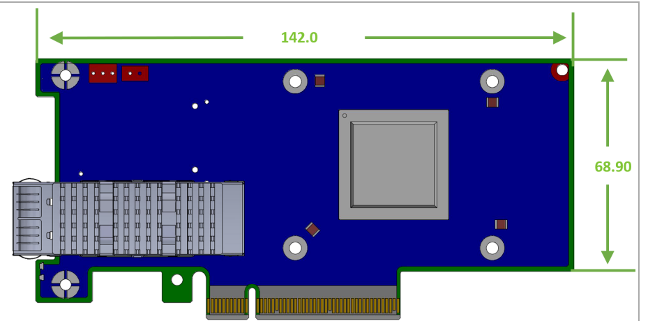
Auxiliary PCIe Connection Card
