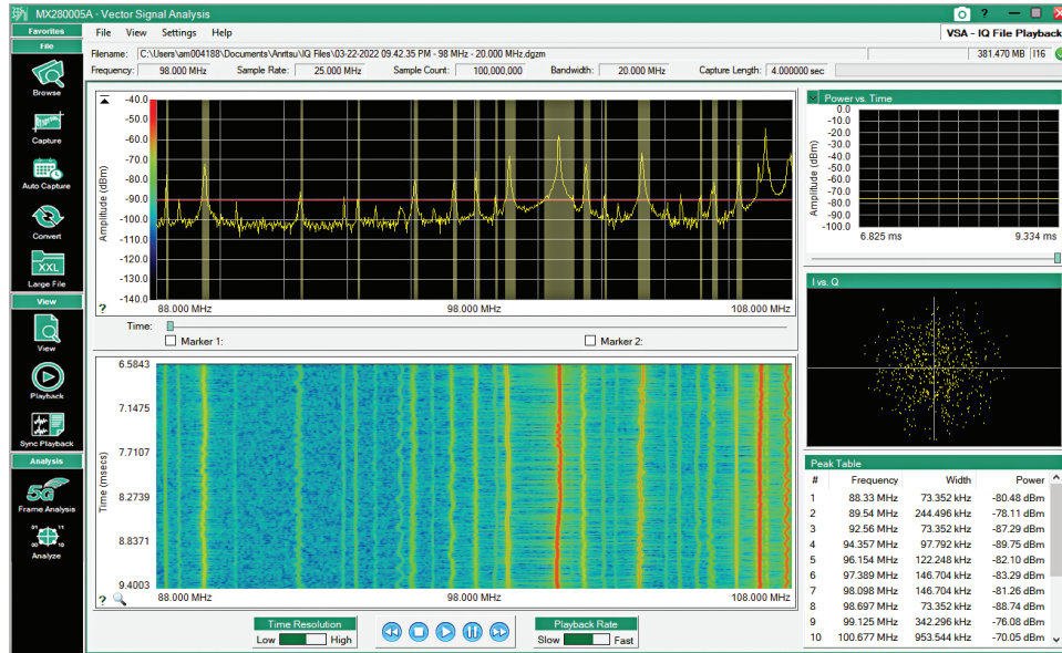
Monitor and Demodulate All FM Transmitters within the Capture Span
