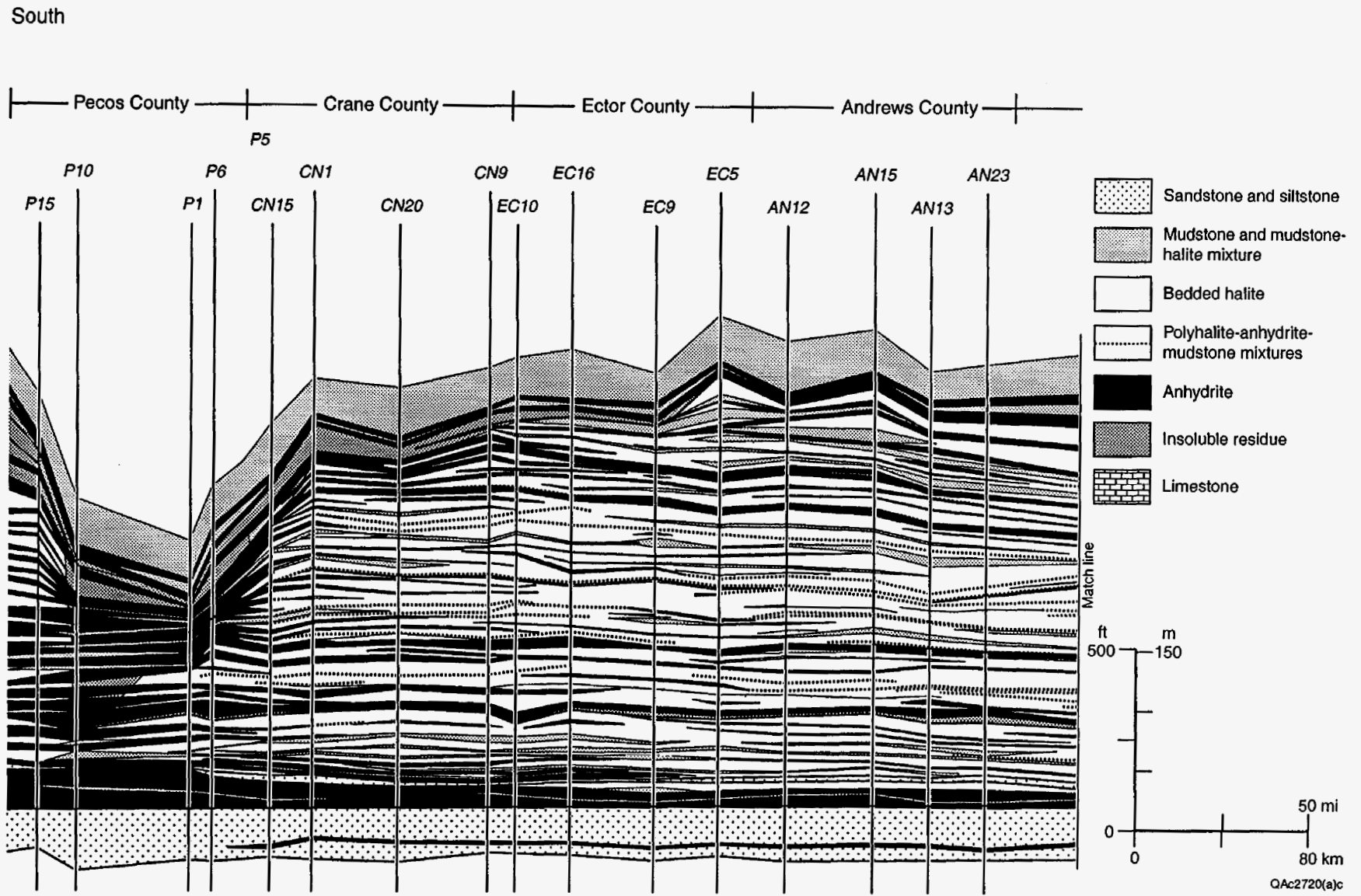
Figure 12. North-south cross section of the Salado Formation and associated units in the Midland Basin. Location of cross section shown in figure 2.
