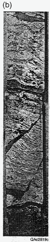
Figure 27 (cont.). Breccia interpreted as a result of formation and collapse of natural salt caverns. (b) Open fractures and rotated blocks above a large collapsed salt cavern, DOE Stone and Webster Sawyer core, 674 ft below datum.
