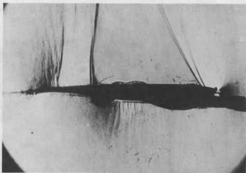
Fig. 4 AIRFOIL 82-06-09 AT M=.83 AND \alpha=1.5^\circ
