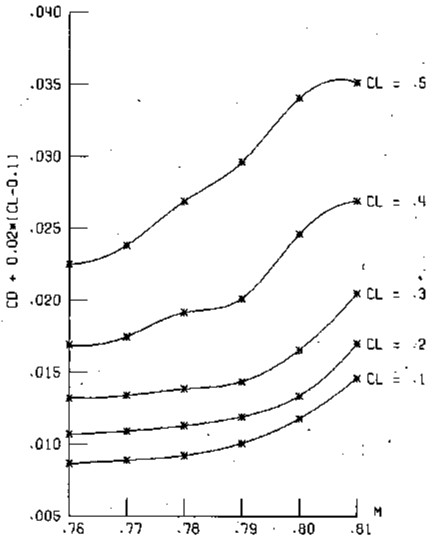
DRAG POLAR FOR AIRFOIL 79-03-12 AT C_L = .1, \dots, .5 AND R = 20 MILLION
