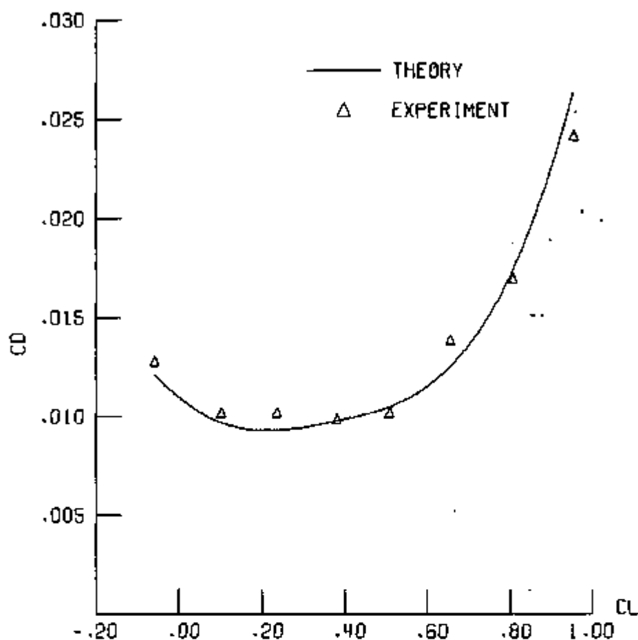
DRAW POLAR FOR AIRFOIL 75-07-15 COMPARING OTTAWA EXPERIMENTAL DATA WITH THEORETICAL ANALYSIS AT M = 0.69 AND R = 20 MILLION
