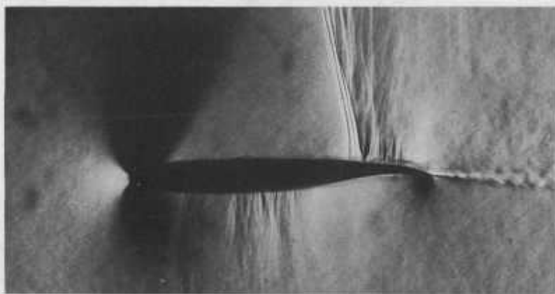
Fig. 3 AIRFOIL 79-07-10 AT M=.84 AND \alpha=2^\circ
