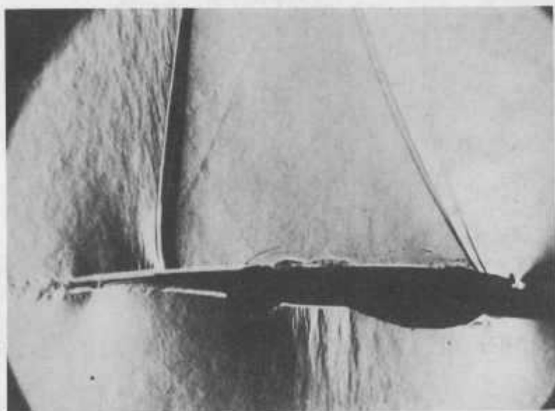
Fig. 5 AIRFOIL 82-06-09 AT M=.84 AND \alpha=1.75^\circ
