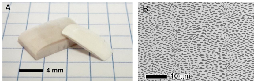
Fig. 8 – Left: Piece of \text{ZrO}_2\text{–MgO} pellet with the laser melted surface (thick sample), with rounded edges. The brownish tinge is an optical effect of the sample microstructure. The thinner slice is the cut and polished solidified layer after acid etching. Right: SEM micrograph of one \text{MgO–ZrO}_2 surface melted eutectic sample after polishing the upper surface. The bright phase is MgSZ, the darker one is MgO. Note that the image shown corresponds to a plane parallel to the larger plate surface, at a distance (some tens of microns) from the upper surface.
