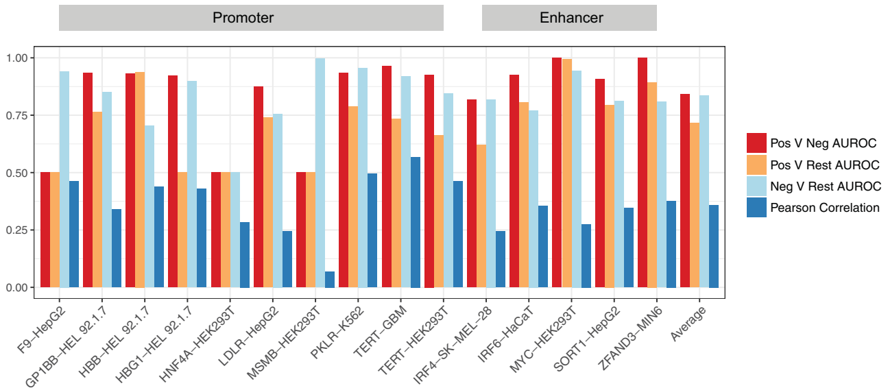
FIGURE 2 Performance across regions. Cell type names are appended at the end of promoter and enhancer regions. The average performance across all regions is also shown. AUROC, area under the receiver operating characteristic
