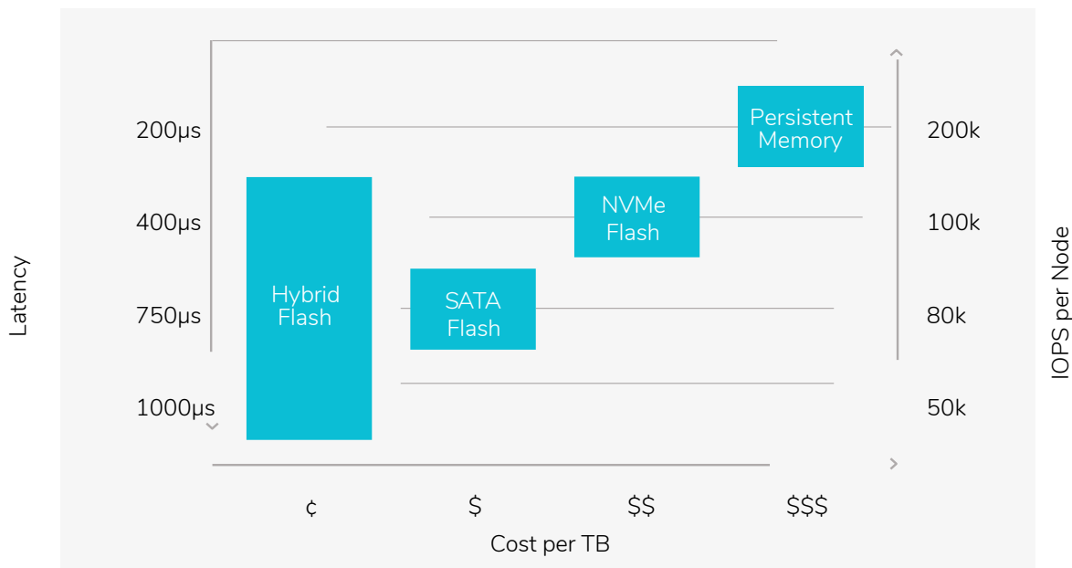
Configurable Datera Node Types by Performance & Capacity
