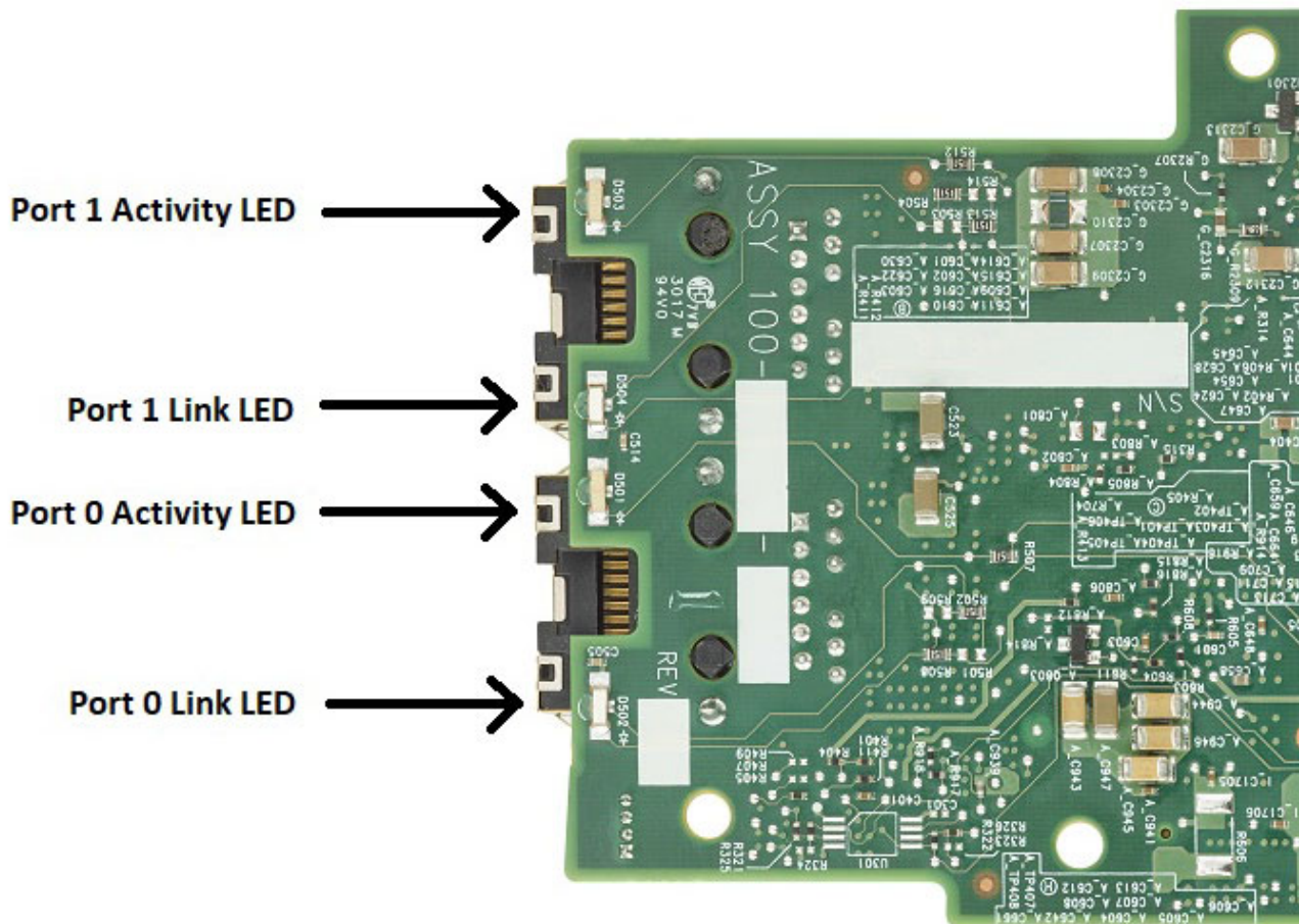
Figure 4: Activity and Link LED Locations
