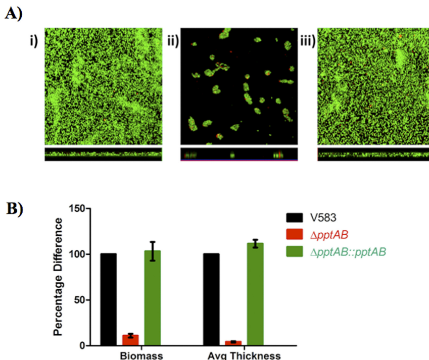
FIG 6 (A) Confocal microscopy biofilm analysis was performed on 1-day-old biofilms of V583 (i), V583 \Delta pptAB (ii), and V583 \Delta pptAB::pptAB (iii). All the strains contain the plasmid pMV158GFP, which provides constitutive expression of GFP. (B) COMSTAT image analysis of biofilms depicted in panel A.
