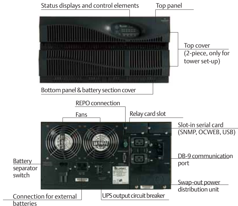
GXT2 rack model (version show: 5U, 4500-6000VA)
