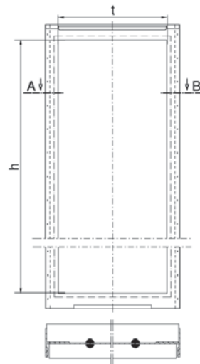
Sealing frame
