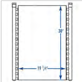
192305 (Northern 192305) RTF 24" INDUSTRIAL OIL COOLER
