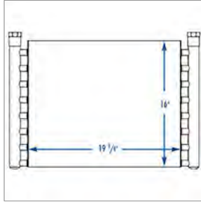
191237 (Northern 191237) RTF 24" INDUSTRIAL OIL COOLER
