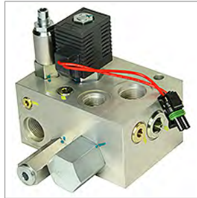
01788116 VALVE ASSY, HYD, 2450 PSI, CP11471-245
