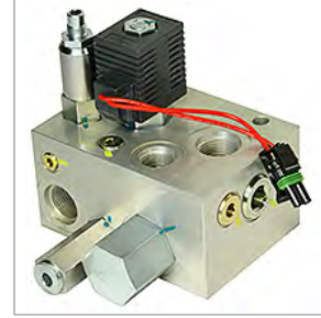
01788082 VALVE ASSY, HYD, 1650 PSI, CP11471-165
