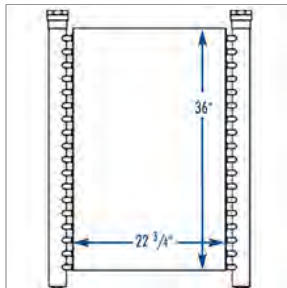
192294 (Northern 192294) RTF 30", 2 ROW INDUSTRIAL OIL COOLER
