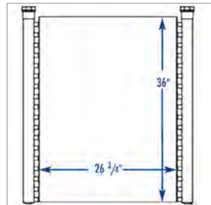
192307 (Northern 192307) RTF 33" INDUSTRIAL OIL COOLER
