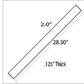
01816180 SPACER, SMOOTH, BLACK, .125 X 2 X 28.30
