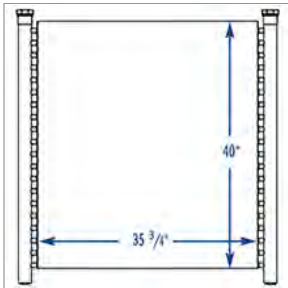
192312 (Northern 192312) RTF 42" INDUSTRIAL OIL COOLER
