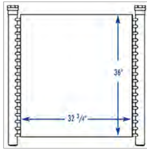
192308 (Northern 192308) RTF 40" 2 ROW INDUSTRIAL OIL COOLER
