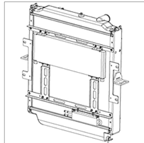
00128295 RADIATOR ASSY,AUX,COMPLETE,COOLING,GM 8.1L BBCV
