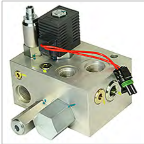
01788090 VALVE ASSY, HYD, 2050 PSI, OP11471-205
