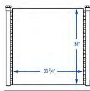
191298 (Northern 191298) RTF 40" INDUSTRIAL OIL COOLER
