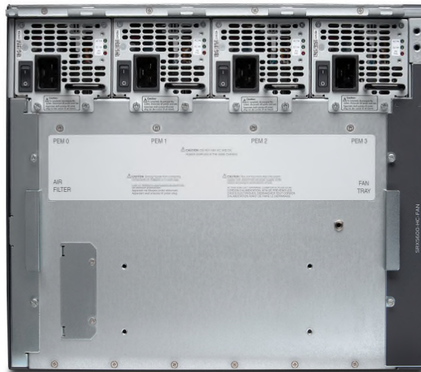
Figure 14 – SRX5600 (Rear)
