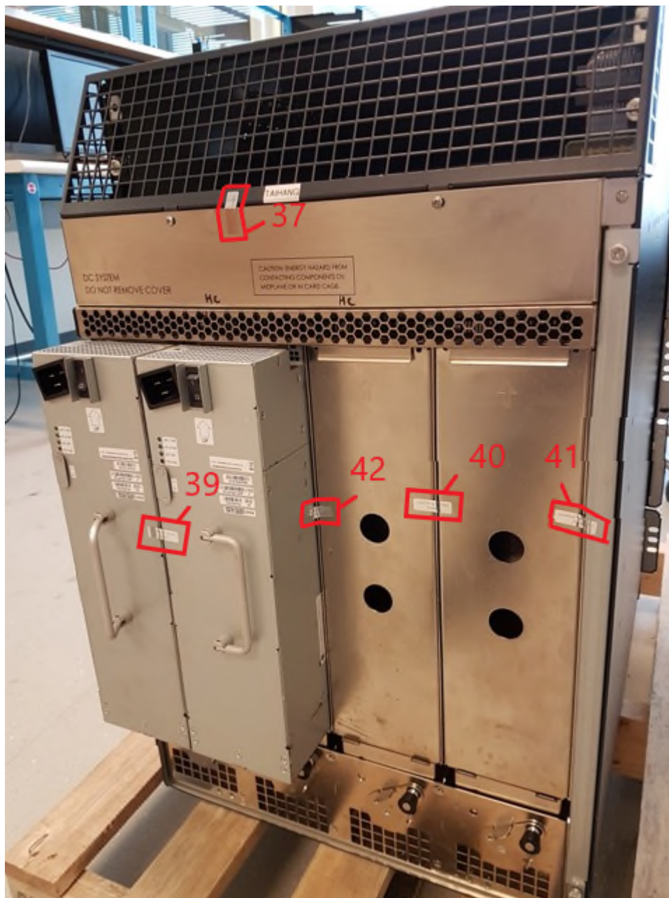
Figure 36 - SRX5800 Tamper-Evident Seal Locations (Rear, Six (6) Seals: TEL 37,39,40-42)
