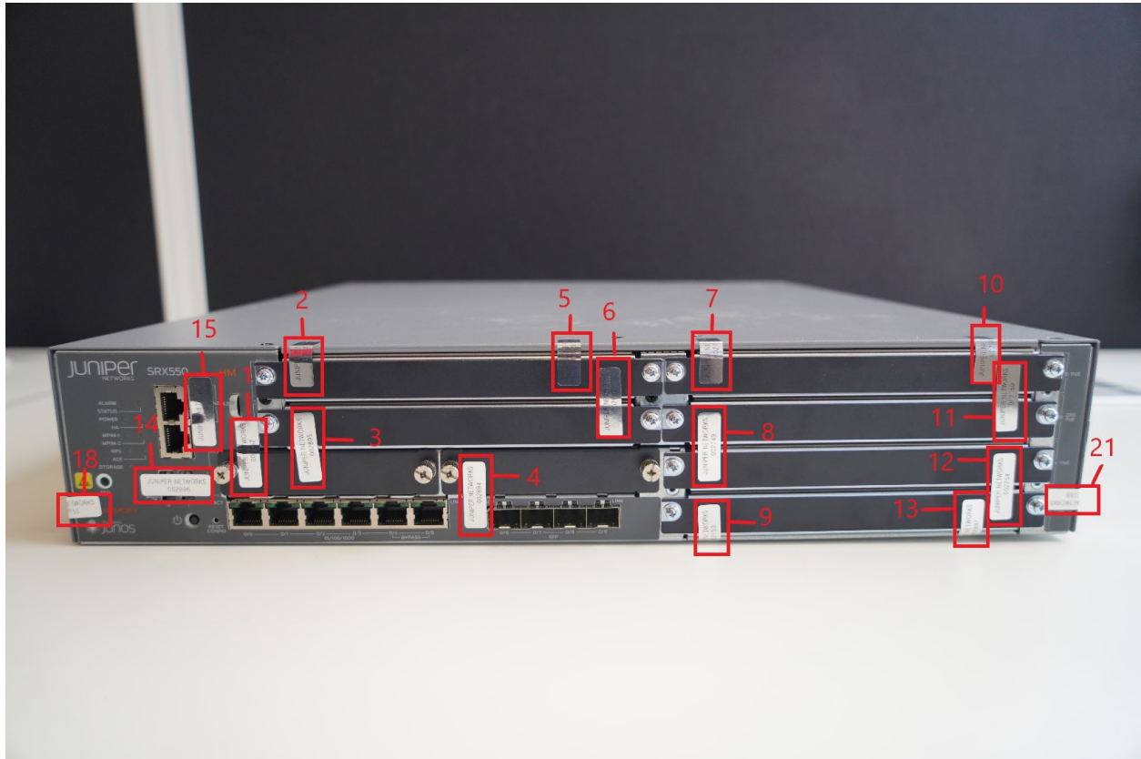
Figure 26 – SRX550M Tamper-Evident Seal Placement (Front, Fifteen (15) Seals: TEL 1-15)
