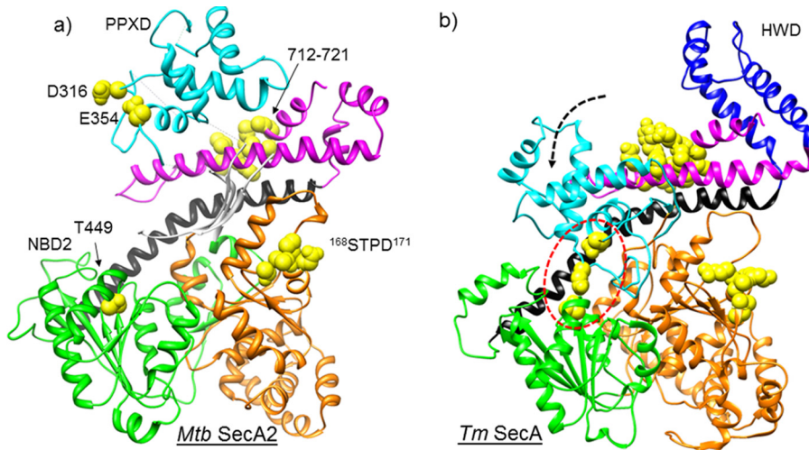
FIG 7 (a) Suppressor mutations from MtSecA2 K129R mapped onto MtSecA2 . Mutations are shown as yellow spheres. (b) Suppressor mutations mapped onto the TmSecA complex with SecYEG (PDB code 3DIN). In the complex with SecYEG, SecA is in the “preprotein clamp closed” conformation, in which PPXD (cyan) is swung down (arrow) to make contact with NBD2 (green). In this conformation, the residues affected by the suppressor mutations in the PPXD and NBD2 domains can be seen to come into contact (circled).
