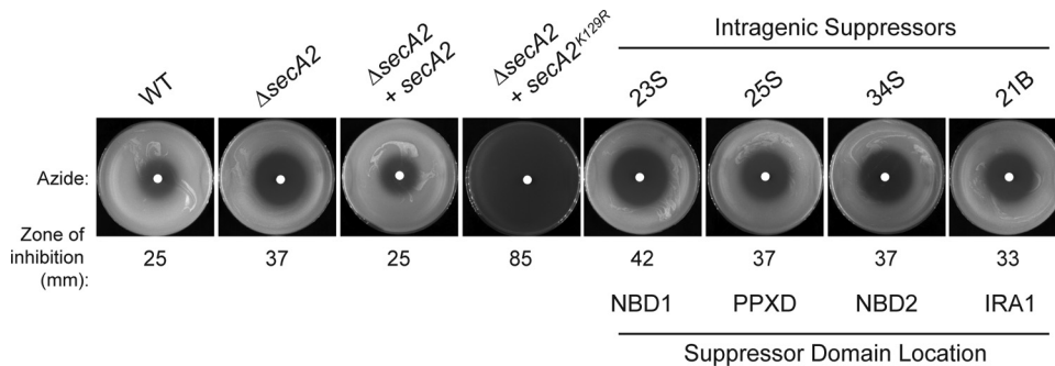
FIG 6 Intragenic suppressors suppress the azide sensitivity phenotype of secA2 K129R . Lawns of the indicated strains were plated and tested for sensitivity to 10 \mu l of 0.15 M sodium azide (applied to a paper disk in the center of the plate) for 2 days at 37°C. Average inhibition was calculated by measuring the diameter of the zone of azide inhibition, and values are the means of three biological replicates. The \Delta secA2 mutant M. smegmatis strain was transformed with plasmids containing either secA2 , secA2 K129R , or a reconstructed intragenic suppressor with the secA2 K129R mutation in combination with an intragenic suppressor mutation located in one of the following domains: NBD1, NBD2, PPXD, or IRA1.
