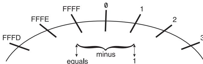
Figure 5. Number Circle Illustration of Memory
