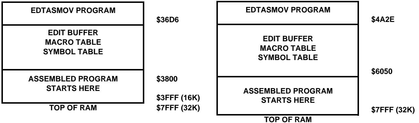
Figure 4. /MO In-Memory Assembly.
