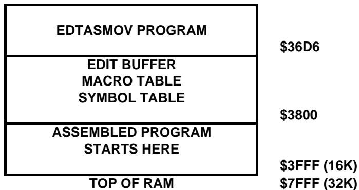
Figure 3. /AO In-Memory Assembly.
