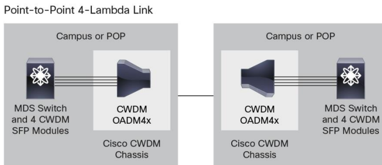
Figure 15. Point-to-Point Architecture (Dual-Fiber Link)
