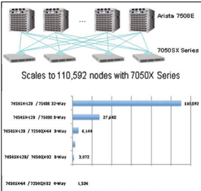
Arista leaf-spine design with L3 ECM
