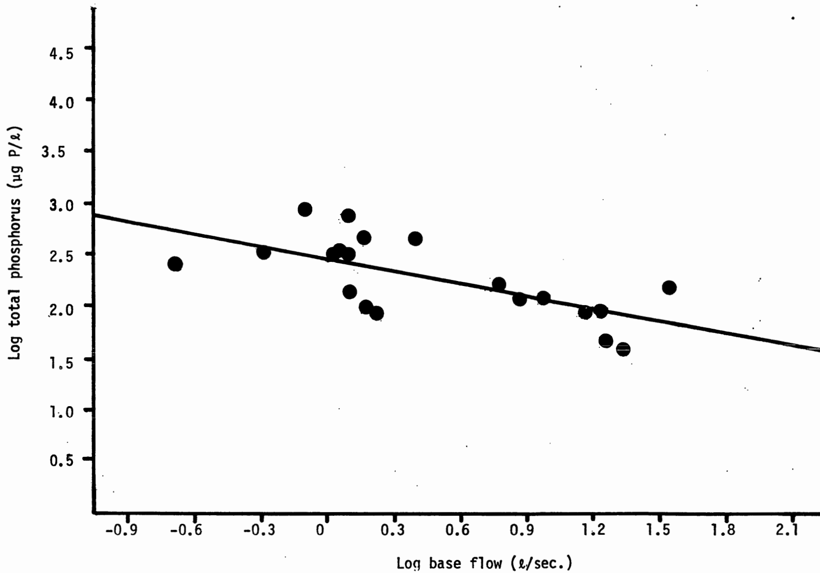
Figure 18. Linear regression of total phosphorus concentration in base flow from basin 101 in the fall of 1971 - 1976.
