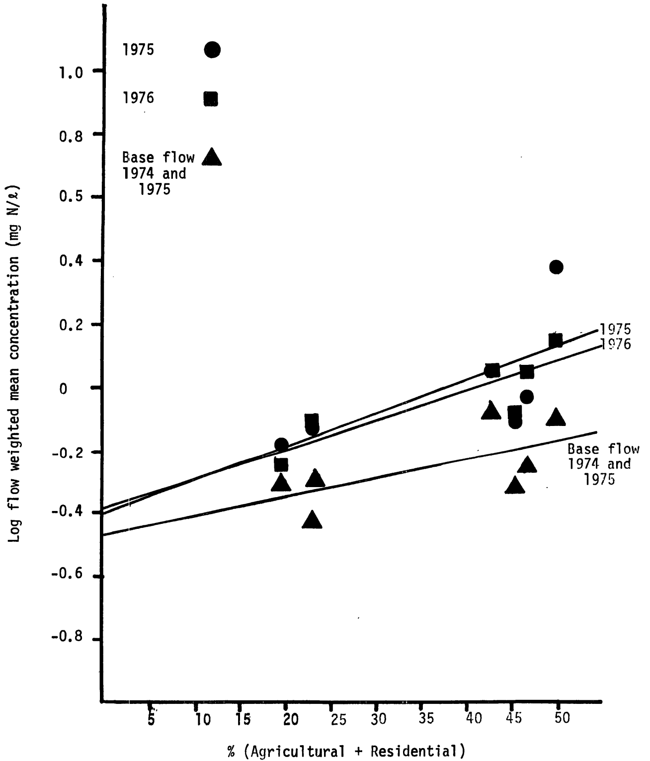
Figure 8. Linear regression of total nitrogen concentration versus percentage of managed land in basins.
