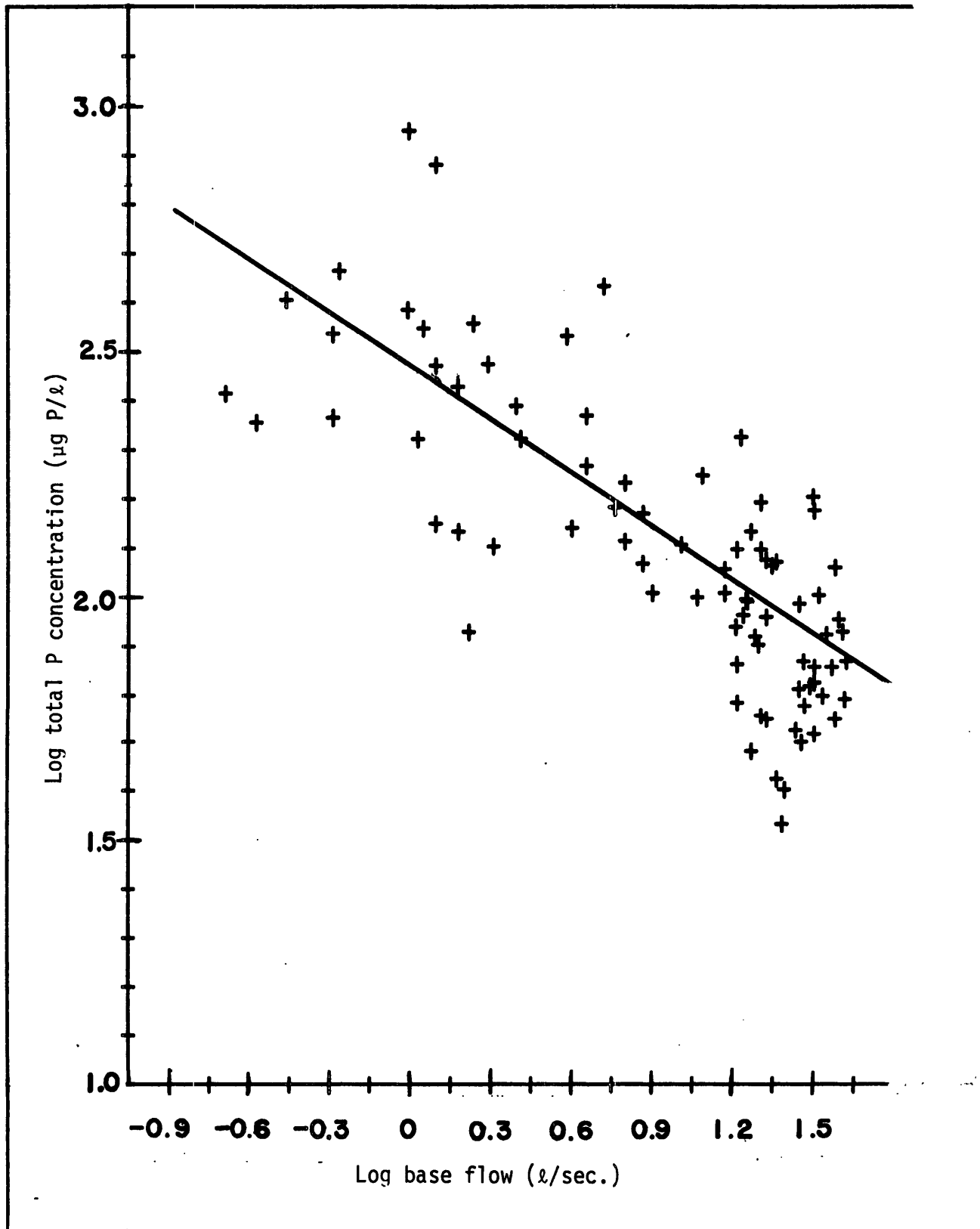
Figure 19. Linear regression of total phosphorus concentration in base flow from basin 101 for the entire period of fall, 1971 to summer, 1976.
