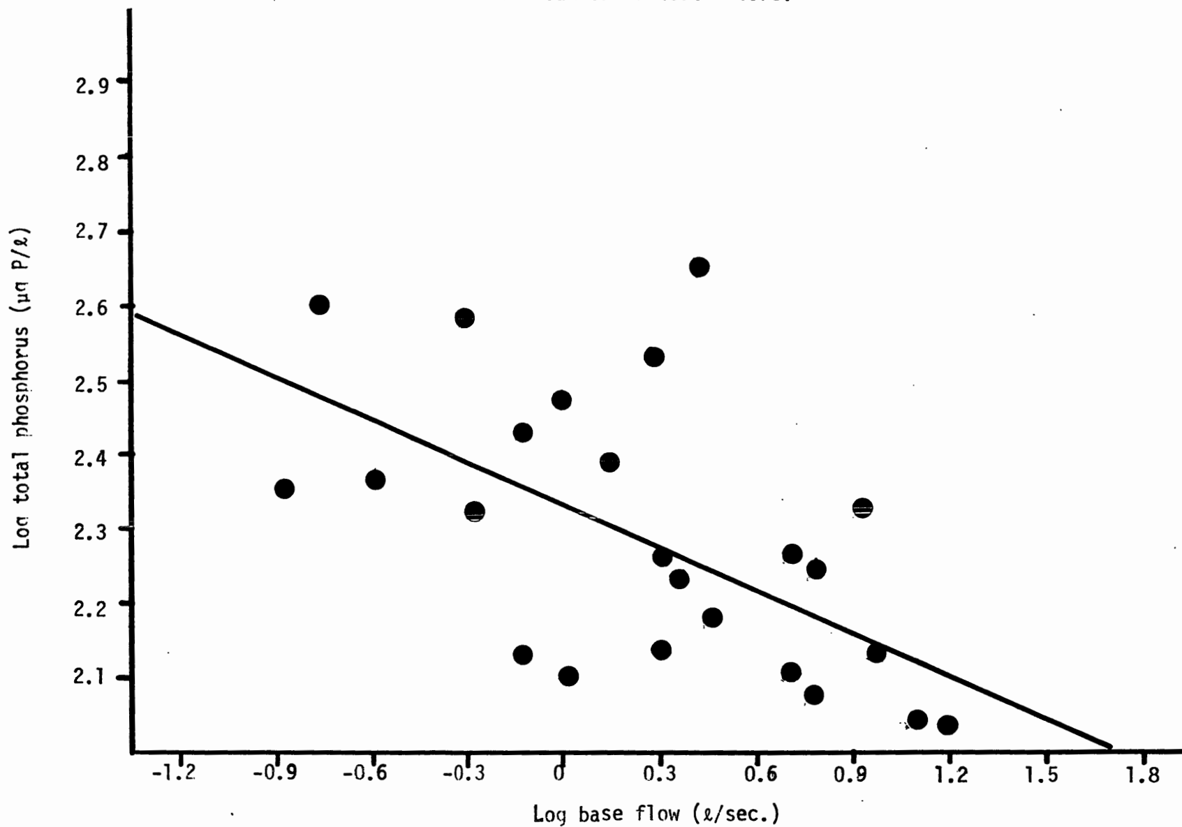
Figure 17. Linear regression of the total phosphorus concentration in base flow from basin 101 in the summer of 1971 - 1976.
