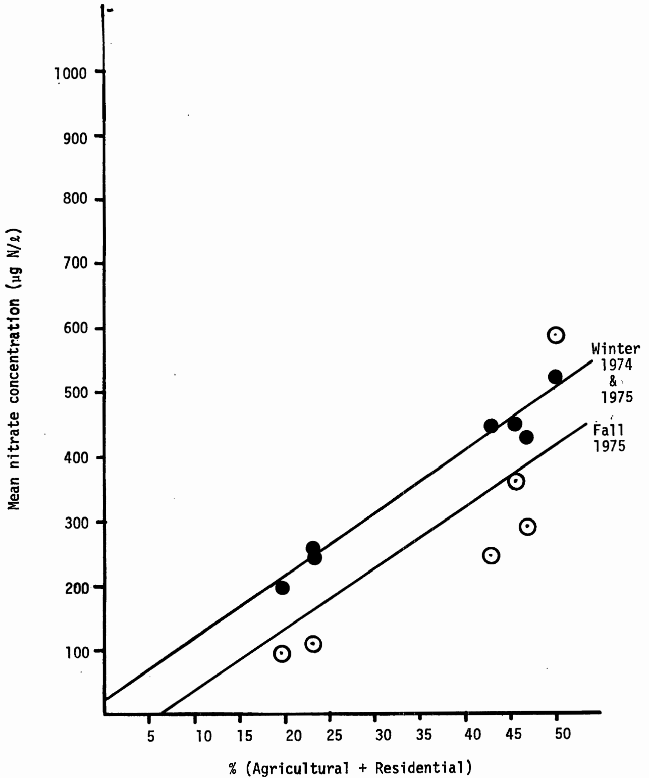
Figure 11. Regression of base flow seasonal mean nitrate concentrations versus percentage of managed land in the basins.
