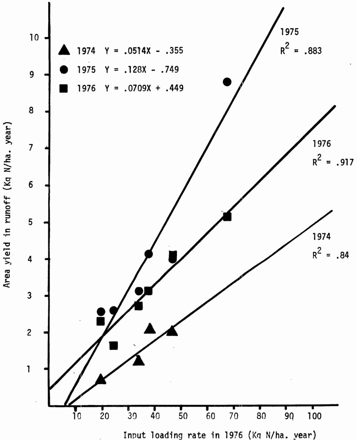
Figure 20. Linear regression of total nitrogen area yields in runoff from various Rhode River basins versus total nitrogen input loadings due to land use practices and rainfall. (Miklas, et al.; in press).
