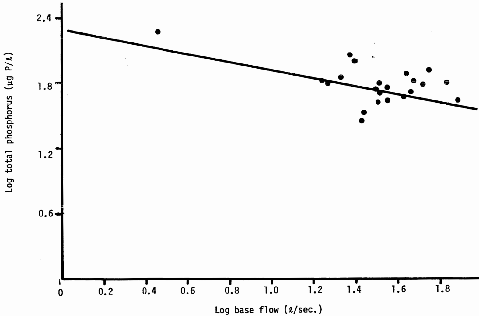
Figure 15. Linear regression of total phosphorus concentration in base flow from basin 101 in the winter of 1971 - 1976.
