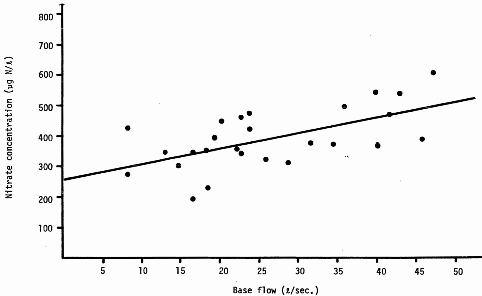
Figure 13. Linear regression of nitrate concentrations in base flow from basin 101 in the spring for 1971 - 1976.
