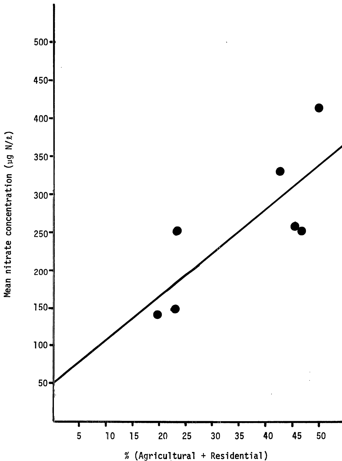
Figure 10. Linear regression of base flow mean annual nitrate concentrations versus percentage of managed land in the basins for 1974 and 1975.
