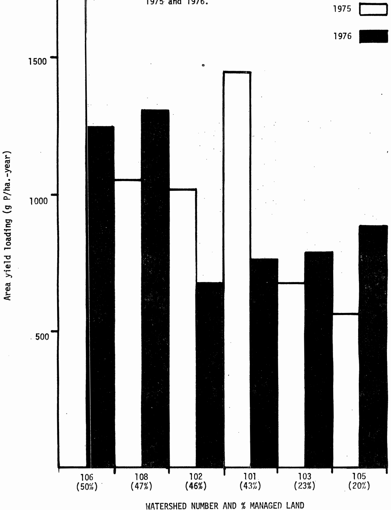
Figure 3. Bar graphs of total phosphorus area yield loading rates from Rhode River watersheds with various degrees of disturbance in 1975 and 1976.
