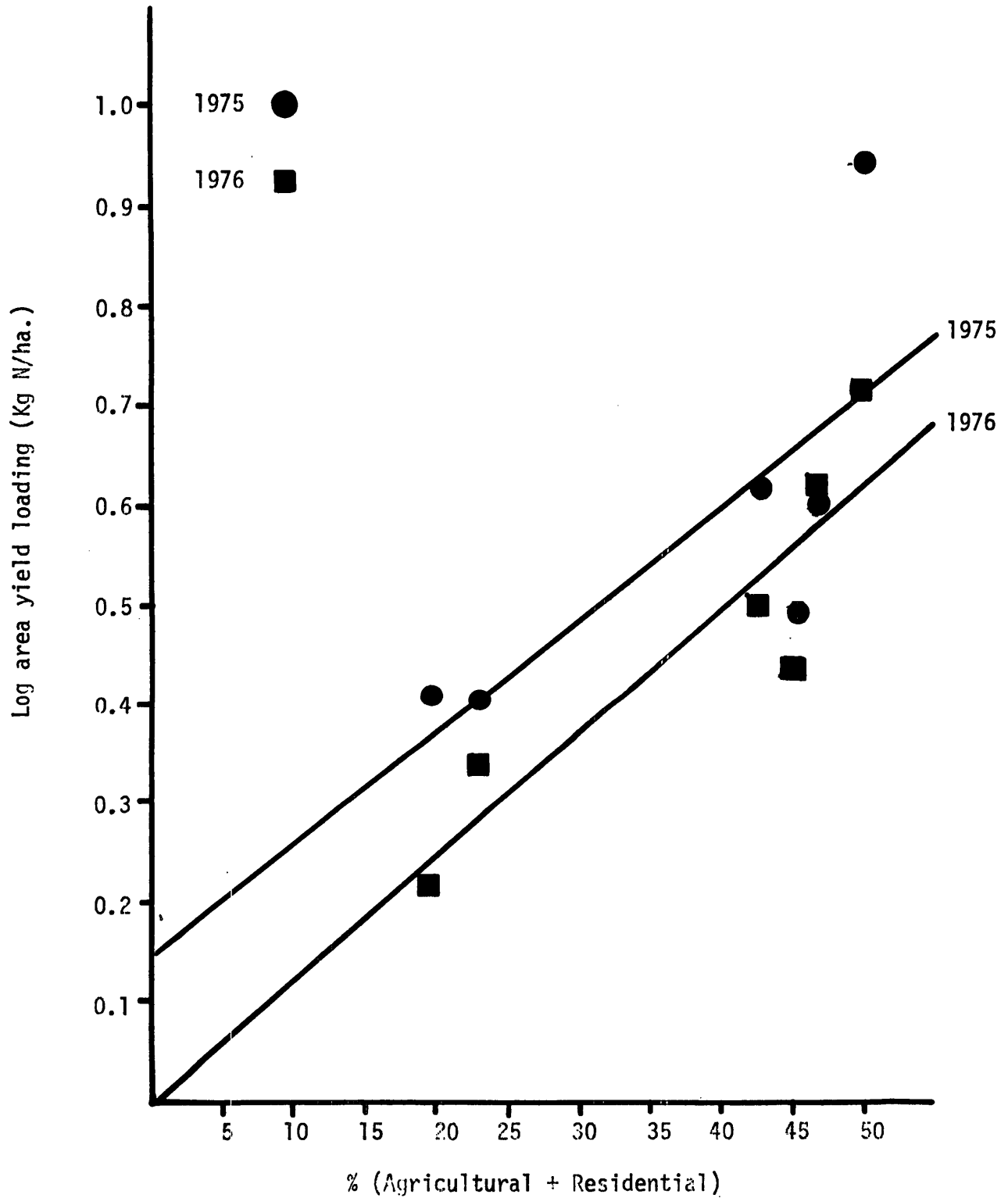
Figure 6. Linear regression of basin total nitrogen area yield loading in runoff versus percentage of managed area in the basins.
