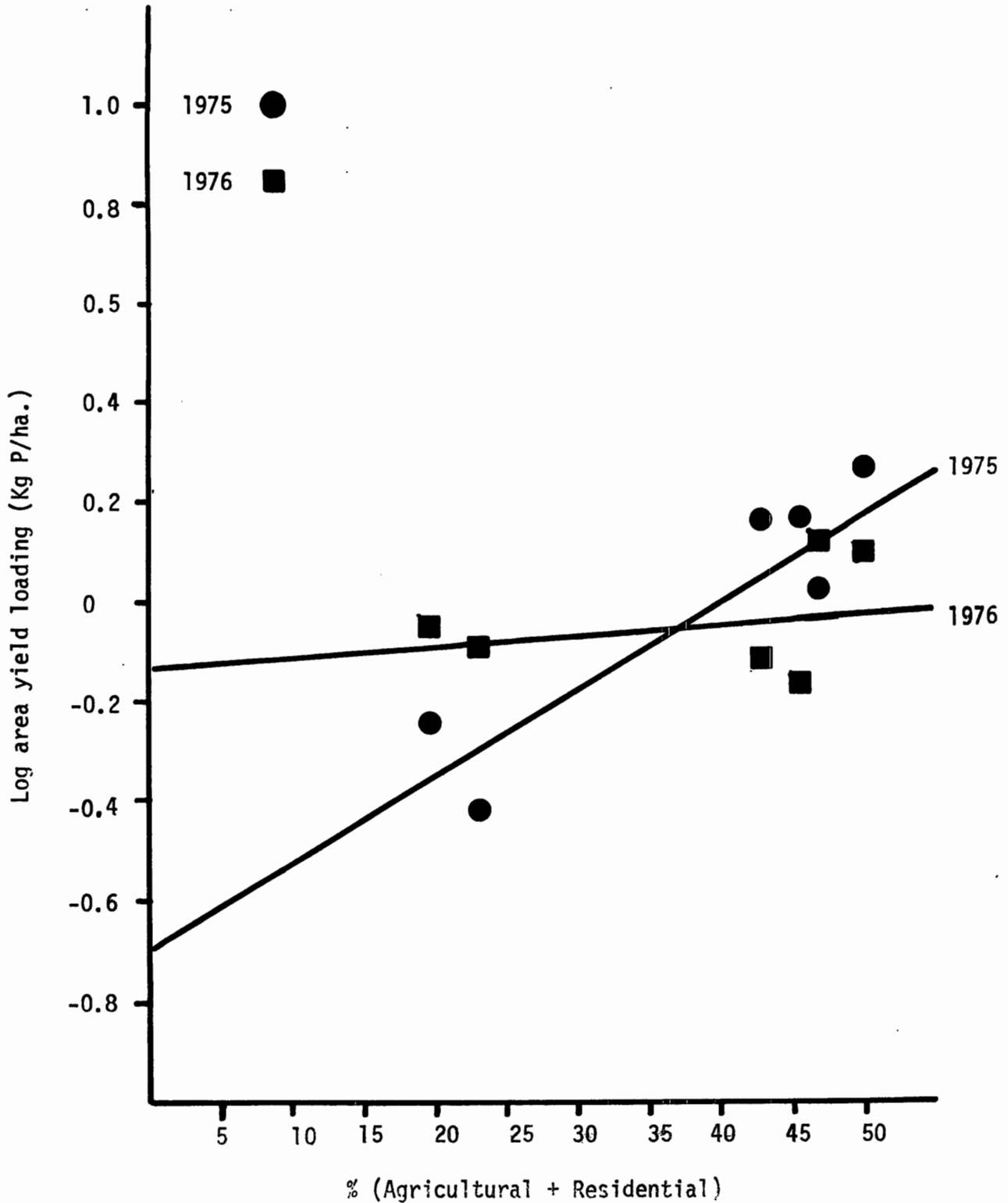
Figure 7. Linear regression of basin total phosphorus area yield loading in runoff versus percentage of managed area in the basins.
