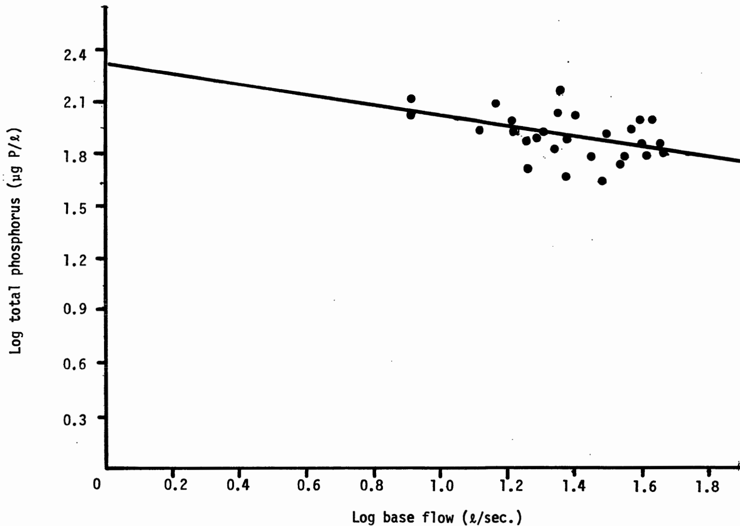
Figure 16. Linear regression of total phosphorus concentration in base flow from basin 101 in the spring of 1971 - 1976.
