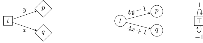
Figure 4.4: Moves in a counter reachability game (left) and the corresponding moves in the \mathbb{Z} -VASS (right).
