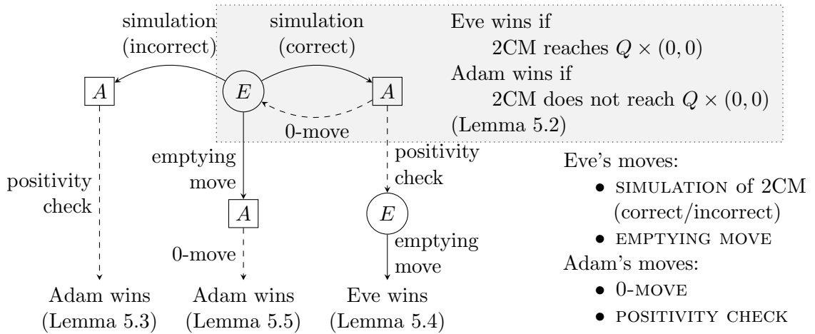
Figure 5.1: Progress of a \mathbb{Z}^2 -VASS game.
