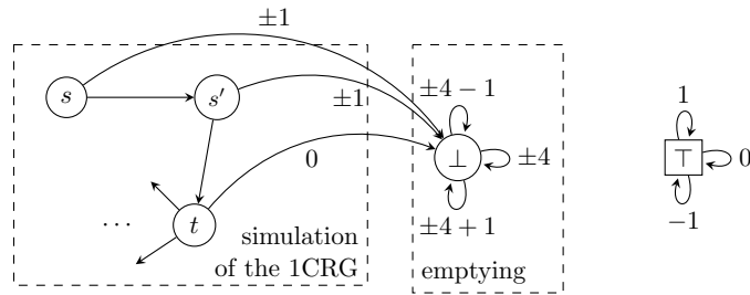
Figure 4.5: An illustration of state transitions of Eve and Adam.
