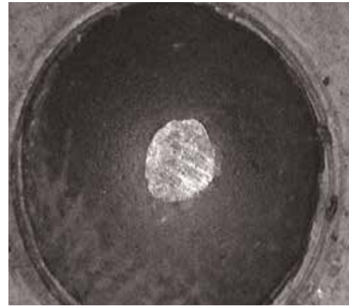
Figure 3: TriCom exhibited excellent wear resistance at 621 °C (1150 °F), surviving 7.9 km (4.9 miles) of sliding wear on a 10mm ball. Wear scar diameter is 0.56 mm.
