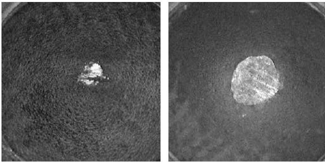
Figure 3: Wear scar on coated spheres from high temperature ball-on-flat wear tests. TriCom-HT (at left) exhibits significantly less wear after 72-hours at 732 °C (1350 °F) than a typical cobalt chromium carbide coating (right). Contact stress was 317 MPa (46 ksi) and total wear distance was 7.9 km (4.9 miles).
