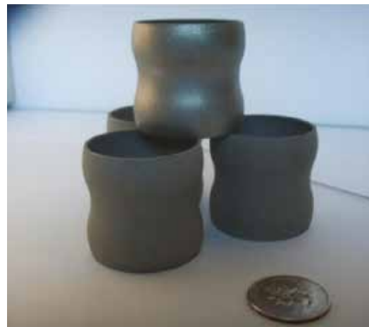
Figure 4: TriCom-HT prevents wear in high load metal to metal sealing applications such as these automotive exhaust manifold couplers.
