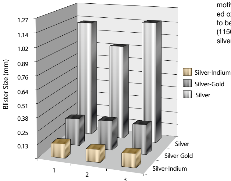
Figure 3: Blister size of Silver, Silver-Gold, and Silver-Indium samples after 500 hours in air at 621 °C (1150 °F).
