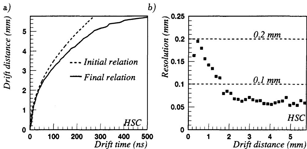
Figure 5.4: a) Drift distance vs. drift time before and after fit procedure. b) Spatial resolution as a function of the drift distance.
