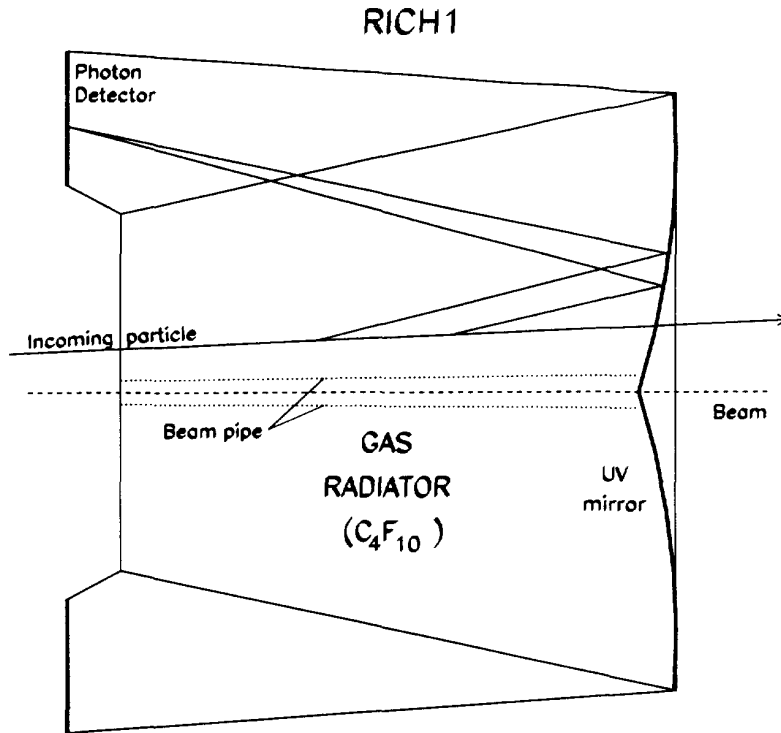
Figure 5.5: Schematic view of the detector RICH1
