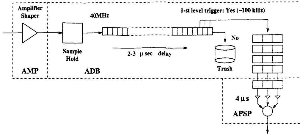
Figure 6.1: The RD20 chip layout.
