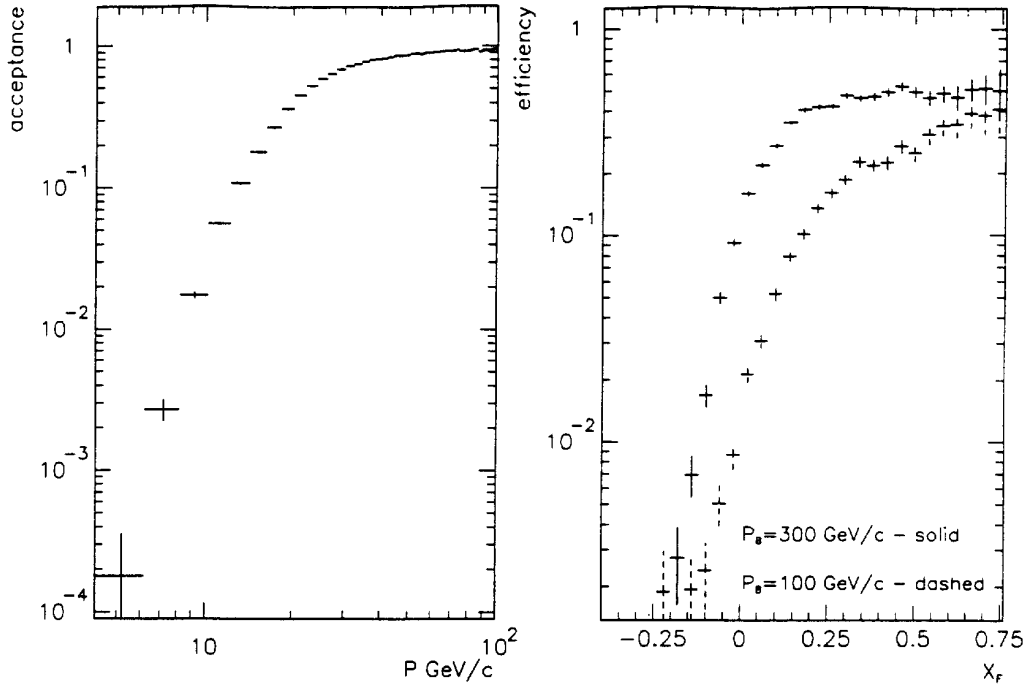
Figure 4.4: The dependence of \epsilon_{acc} on the longitudinal momentum averaged for all processes considered; the dependence of \epsilon_{MC} on the x_F for beam energies of 300 and 100 GeV.
