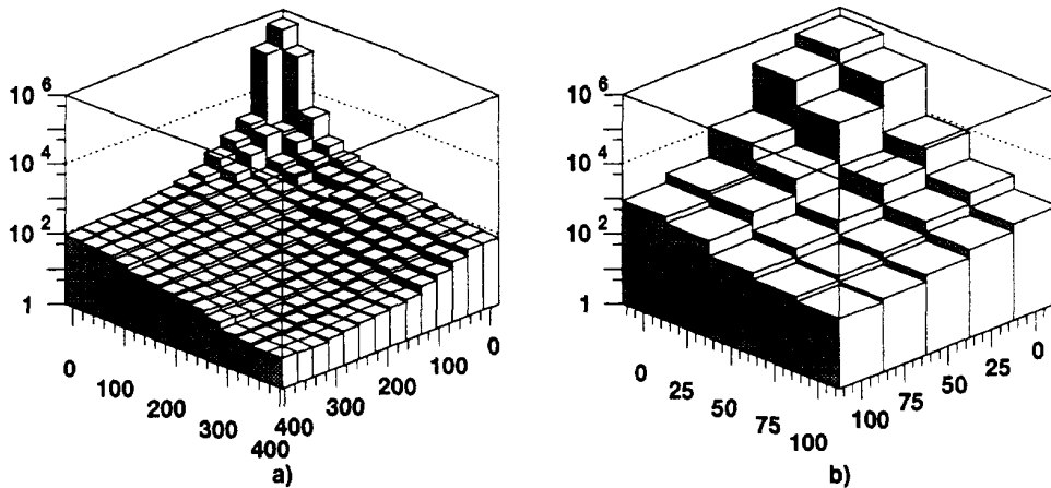
Figure 5.17: The beam halo normalised to 1 \text{ cm}^2 and 10^7 muons, in a 400 \times 400 \text{ mm}^2 (a) and a 100 \times 100 \text{ mm}^2 quadrant (b).
