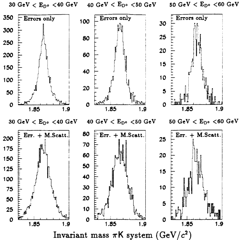
Figure 5.25: Invariant mass distribution of the \pi K from D^0 decays for three different D^0 energy ranges, when the \pi or/and the K enter the SAS. The upper row refers to the case where location errors only are taken into account. The second row refers to the “full” case (both multiple scattering and location errors are there).
