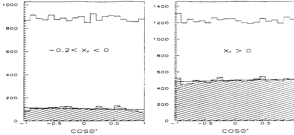
Figure 3.14: A decay angular distribution for the target fragmentation region ( -0.2 < x_F < 0 ) (left) and the current fragmentation region ( x_F > 0 ) (right). The solid lines correspond to the generated distributions and the hatched area to accepted events.
