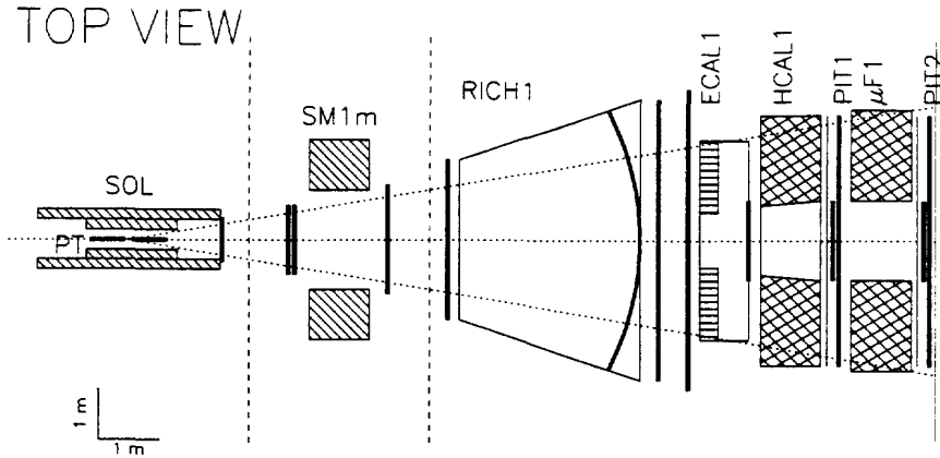
Figure 2.3: Schematic layout of the large angle spectrometer for the muon beam programme.
