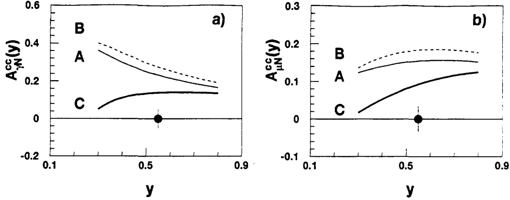
Figure 3.6: a) Asymmetry A_{\gamma N}^{cc} and b) asymmetry A_{\mu N}^{cc} , for open charm as a function of y . The curves refer like in Fig. 3.1 to the three sets of \Delta G from Ref. [4]. The projected precision of the measurement in the range 0.35 < y < 0.85 is indicated by the error bars of the data points shown at A = 0 .
