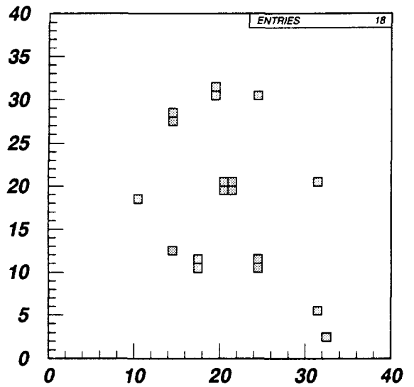
Figure 5.10: Cherenkov rings on RD26 photon chambers, generated by 3 GeV/c pions and 3 GeV/c protons crossing 10.5 mm of C_6F_{14} freon radiator.
