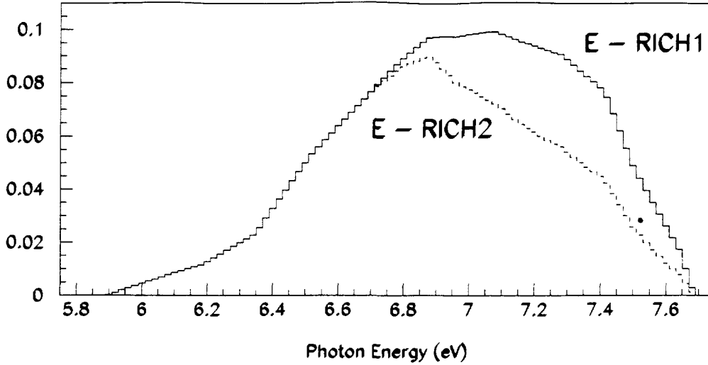
Figure 5.12: E for RICH1 and for RICH2 versus photon energy.
