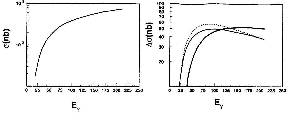
Figure 3.3: Charm photoproduction cross sections as a function of the photon energy E_\gamma . a) unpolarised cross section \sigma^{\gamma N \rightarrow c\bar{c}X} , b) polarised cross section \Delta\sigma^{\gamma N \rightarrow c\bar{c}X} . For the different lines see Fig. 3.1.
