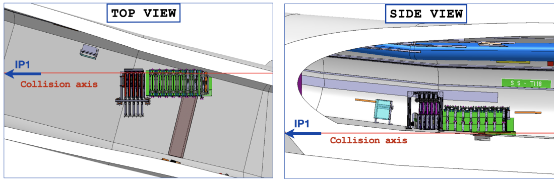
Figure 4: Side and top views of the SND@LHC detector in the TI18 tunnel [2].
