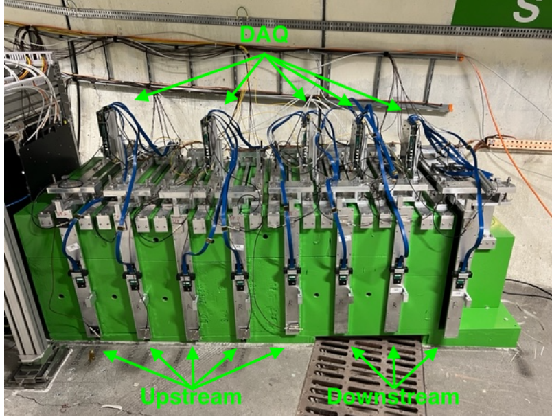
Figure 16: Picture of the hadronic calorimeter and muon system installed in TI18.
