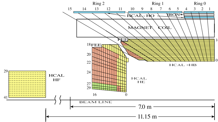
Figure 2.8: Cross sectional view of the CMS hadronic calorimeter (HCAL) detector in the r-z plane, depicting the positioning of the various detector segments relative to the beam line and the solenoid magnet. The HCAL is symmetric around r = 0 , so only the top half is shown. The figure adapted from [68].
