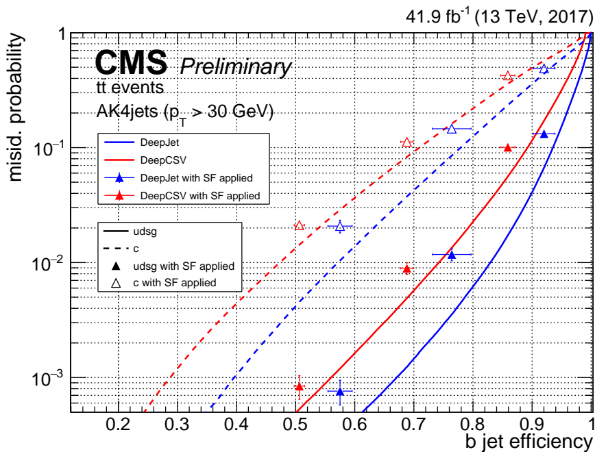
Figure 4.4: Misidentification probability (in log scale) for jets originating from c quarks (dashed lines) or light quarks and gluons (solid lines) as a function of the b-tagging efficiency for both DeepCSV and DeepJet taggers. The corrected mistag/efficiency and its uncertainty for the loose, medium and tight working points are also included. Figure adapted from [138].
