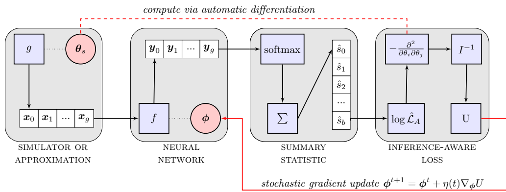
Figure 6.1: Learning inference-aware summary statistics (see text for details).
