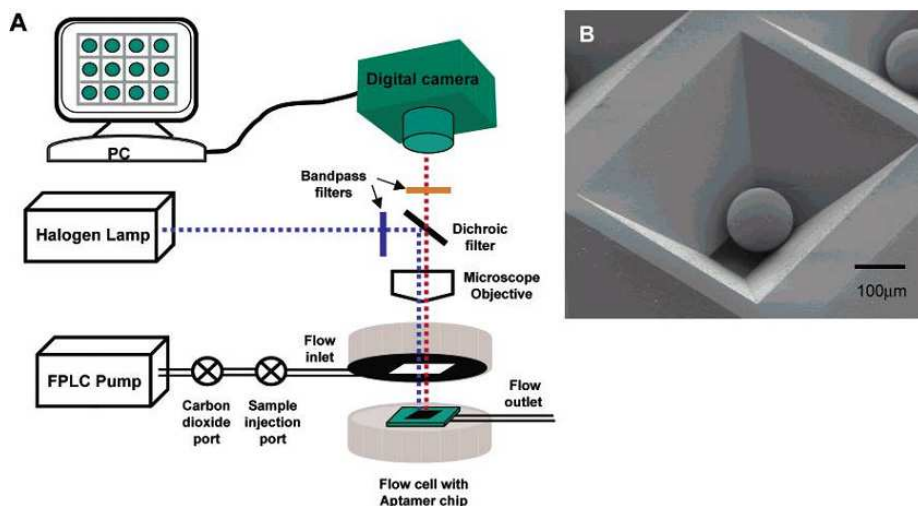
Fig. 11. Detection systems. (A) The electronic tongue setup contains a fluid delivery system, fluorescence microscope, digital camera, flow cell in which the aptamer chip will be loaded, and computer for data analysis. (B) Close-up look at a bead in a rectangular-shaped micro-machined well of the aptamer chip. Reprinted from ref. 40 with permission by the Royal Society of Chemistry.
