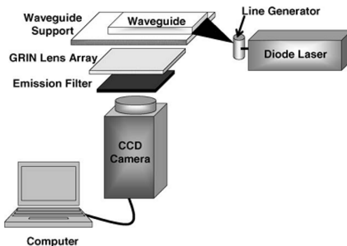
Fig. 8. Schematic of the NRL array biosensor. Reprinted from ref. 22 with permission by the Elsevier.
