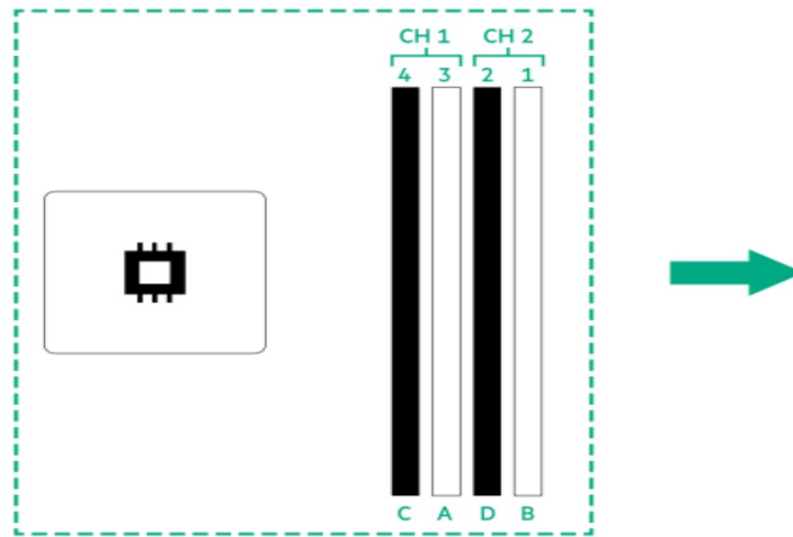
DIMM slot and configuration diagram
