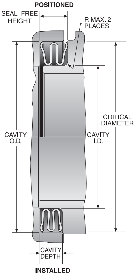
JEE E-SEAL, EXTERNAL PRESSURE
