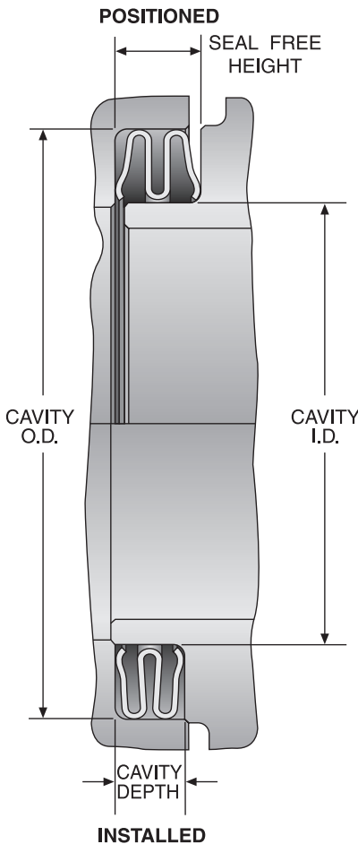
JEI E-SEAL, INTERNAL PRESSURE
