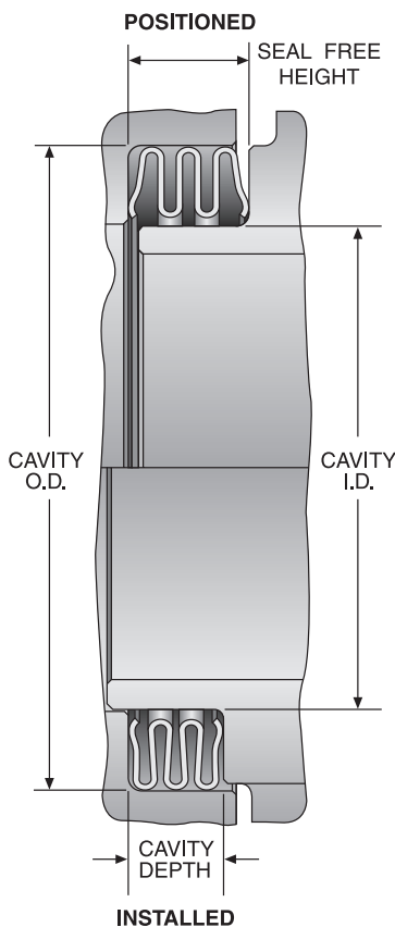
JW E-SEAL, INTERNAL PRESSURE
