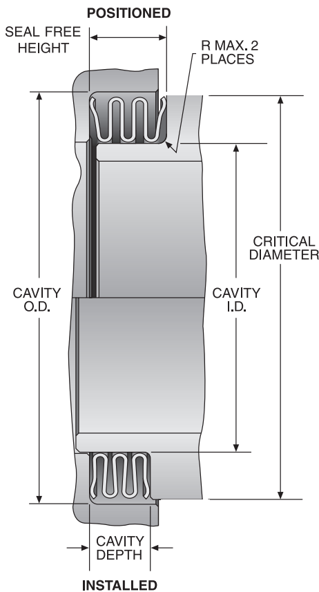
JWE E-SEAL, EXTERNAL PRESSURE
