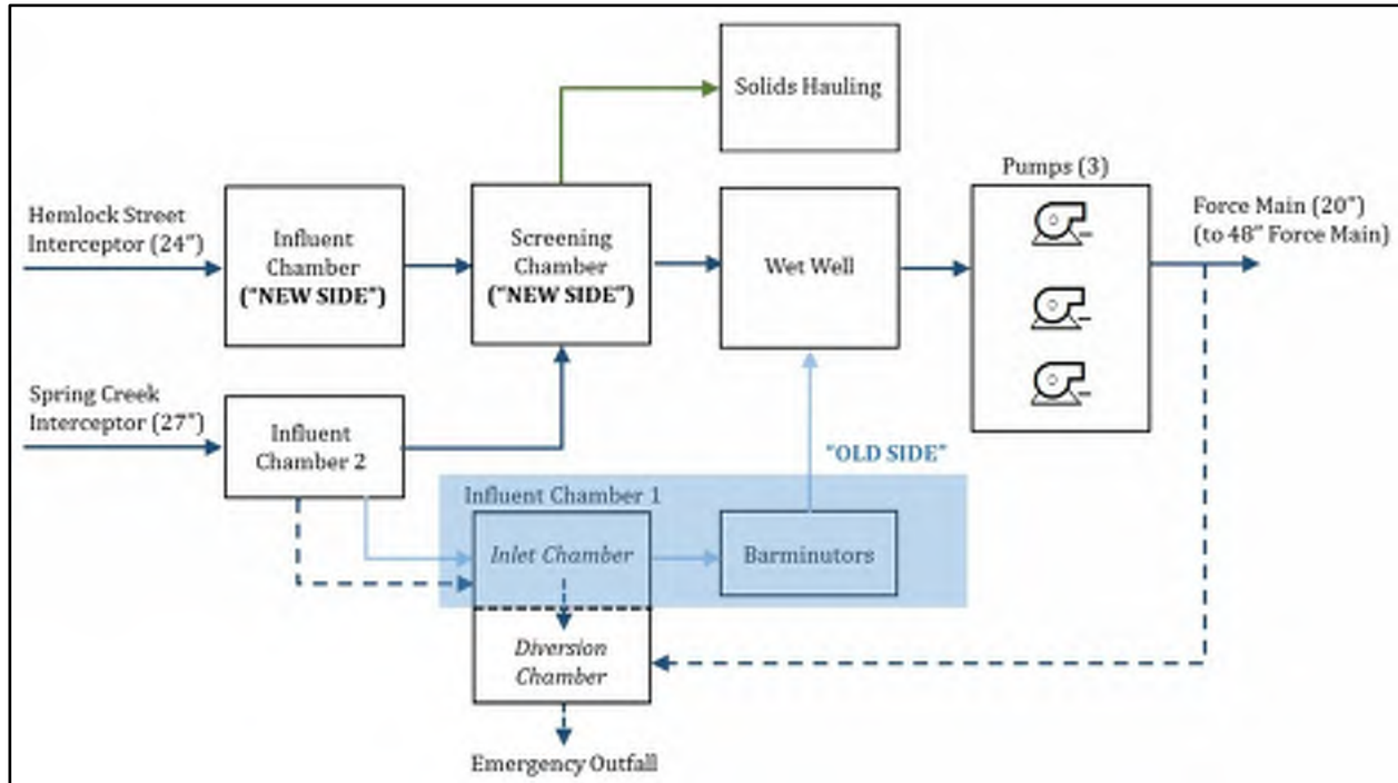
Figure 4.3-8 Spring Creek Pump Station Flow Schematic
