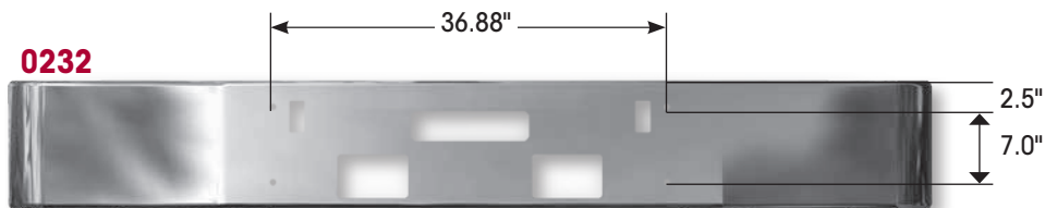
Freightliner FLD 112
