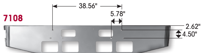
Ford Conventional LTL 9000 — Step holes and four square light holes.
