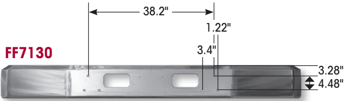
Ford OEM 8000 and 9000 Batwing Aero FF7131 has bolt holes for air dam.
