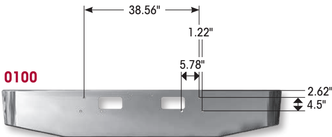
Ford L-Series conventional fits LN-LT-LTN 800, 900, 8000 and 9000 (Tow holes only). Fits trucks with 6V92 Detroit engine or 300 Cummins engine 1988 or newer (Axle forward only).
