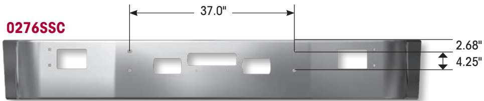
Freightliner FLD 120
