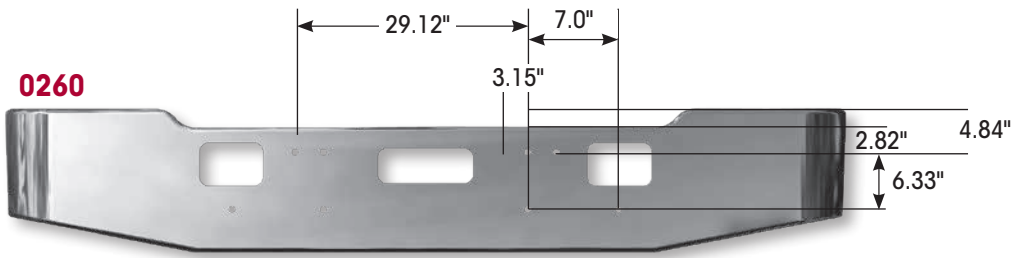
Freightliner FLC-112
