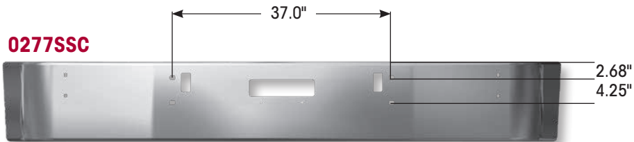
Freightliner FLD 112 with step and tow holes
