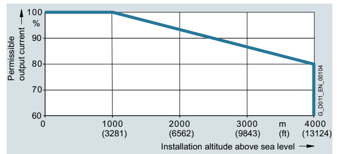
Permissible output current as a function of the installation altitude for PM250 Power Modules, frame sizes FSC to FSF
