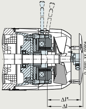
Fig. 3 Brake and rotary pulse encoder (on cover), order codes F01/F04 + G04/G05/G06/G11/G12 [optionally with manual release, order code F50 ; G11, G12 protective cover as standard]
