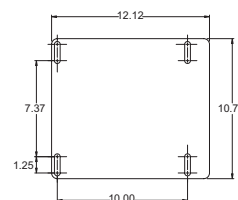
Mounting Base Dimensions (in.)
