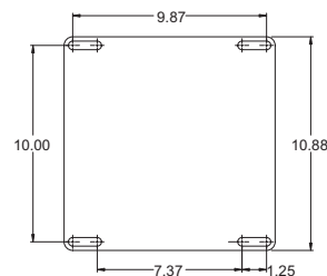
Mounting Base Dimensions (in.)
