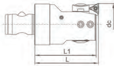
Forward boring
