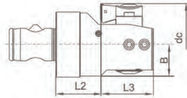
back boring
