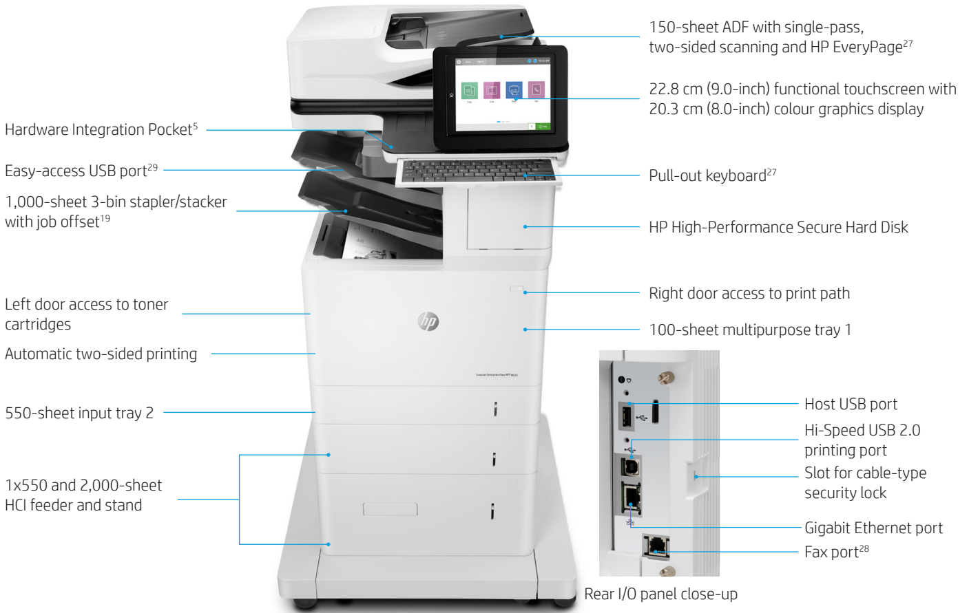
Front view
