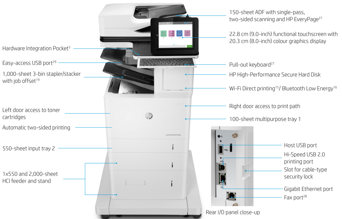
Front view
