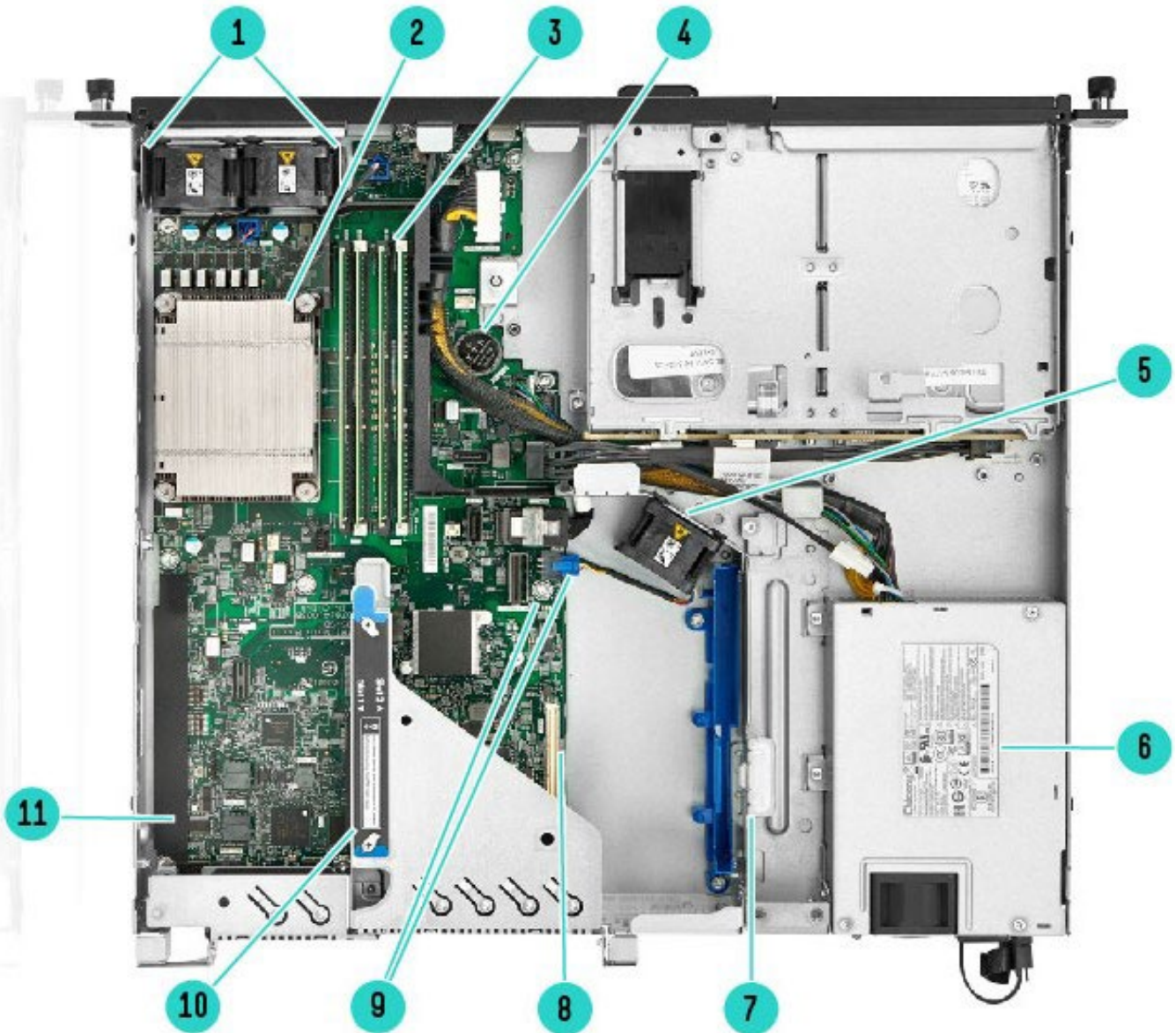
Internal View - Standard for all 2LFF DL20 Gen10 Plus
