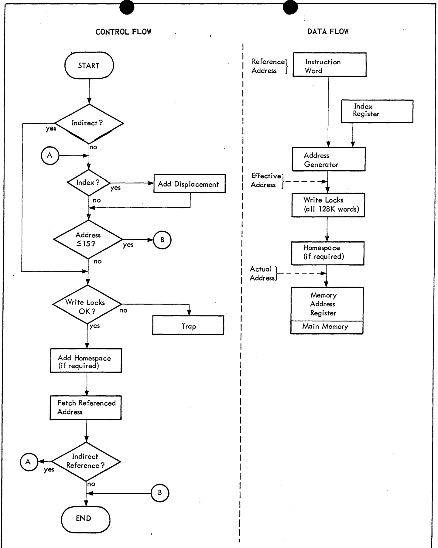
Figure 4. Addressing Logic
