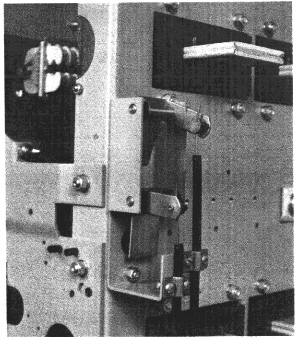
Mechanical Interlock
