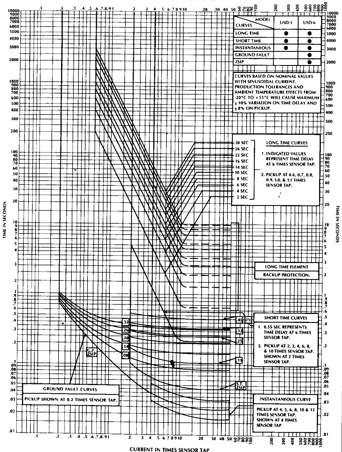
TIME-CURRENT CHARACTERISTICS
